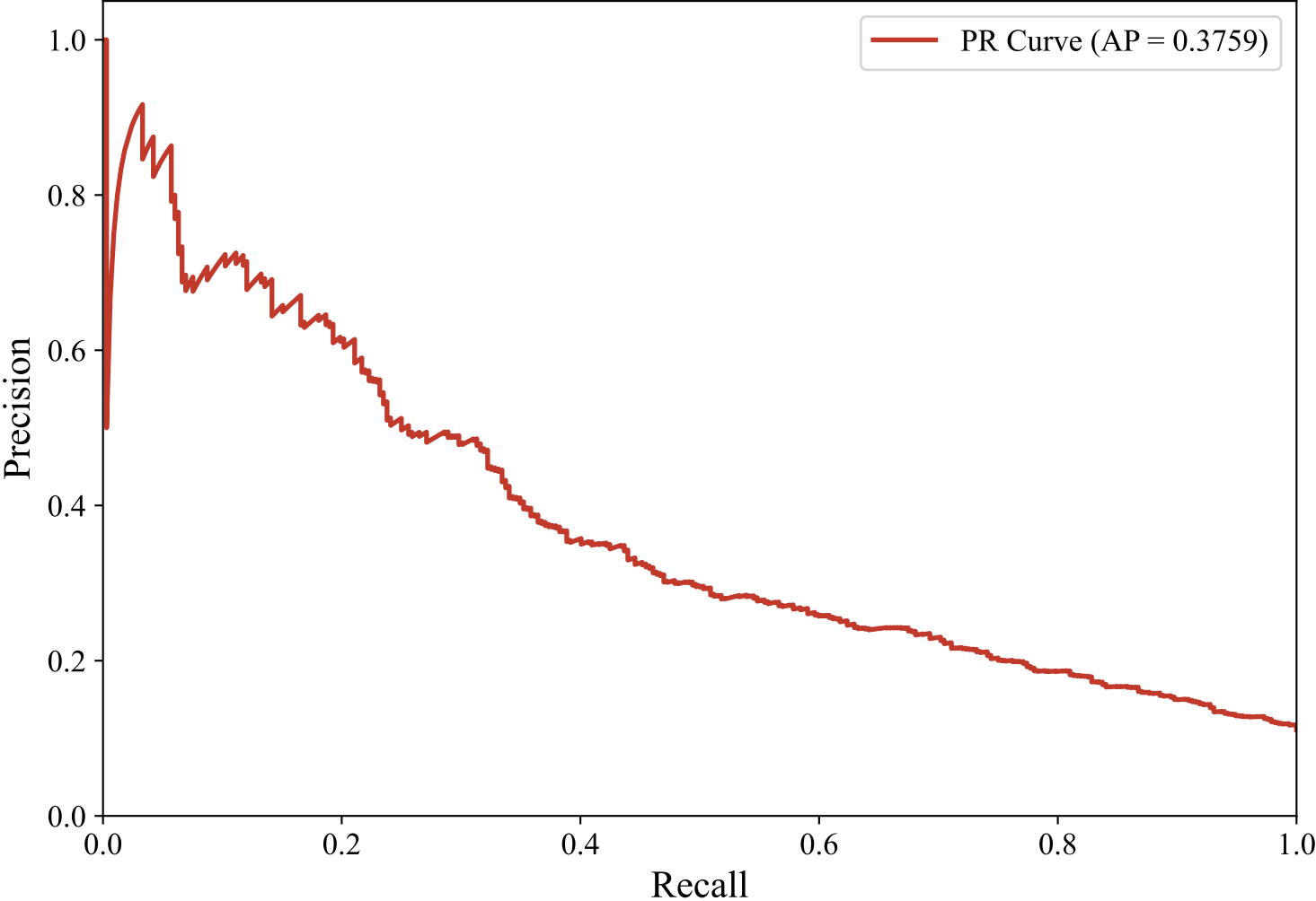
Precision-Recall Curve — GERMAN_MANUAL (paraphrase-multilingual-MiniLM-L12-v2, Voting_Ensemble)
