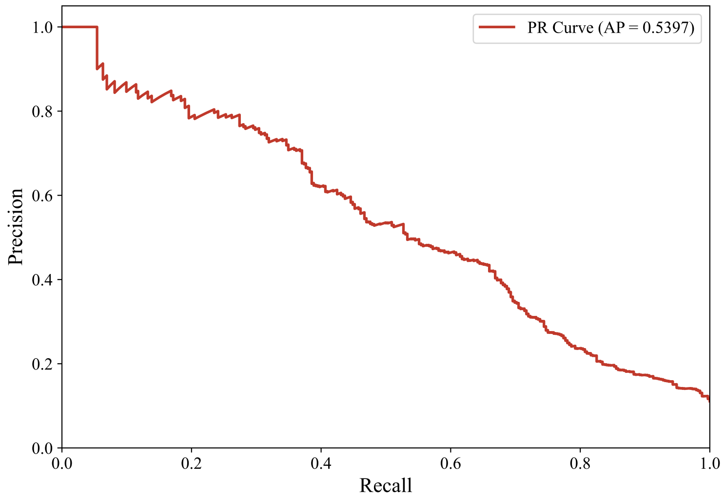
Precision-Recall Curve — GERMAN_MANUAL (snowflake-arctic-embed-l-v2.0, LightGBM)
