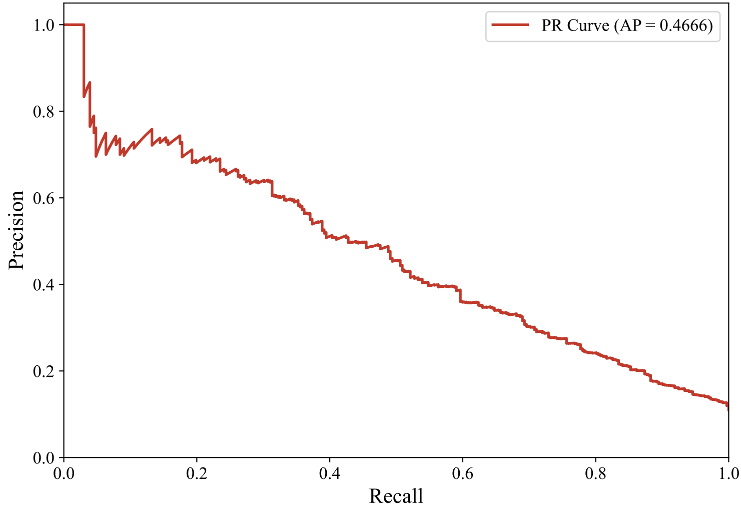
Precision-Recall Curve — GERMAN_MANUAL (snowflake-arctic-embed-l-v2.0, Random_Forest)
