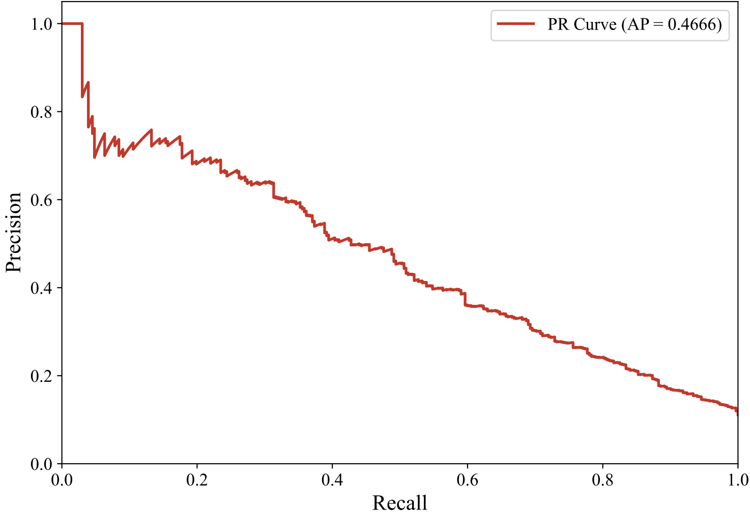
Precision-Recall Curve — GERMAN_MANUAL (snowflake-arctic-embed-l-v2.0, Random_Forest_Optimized)
