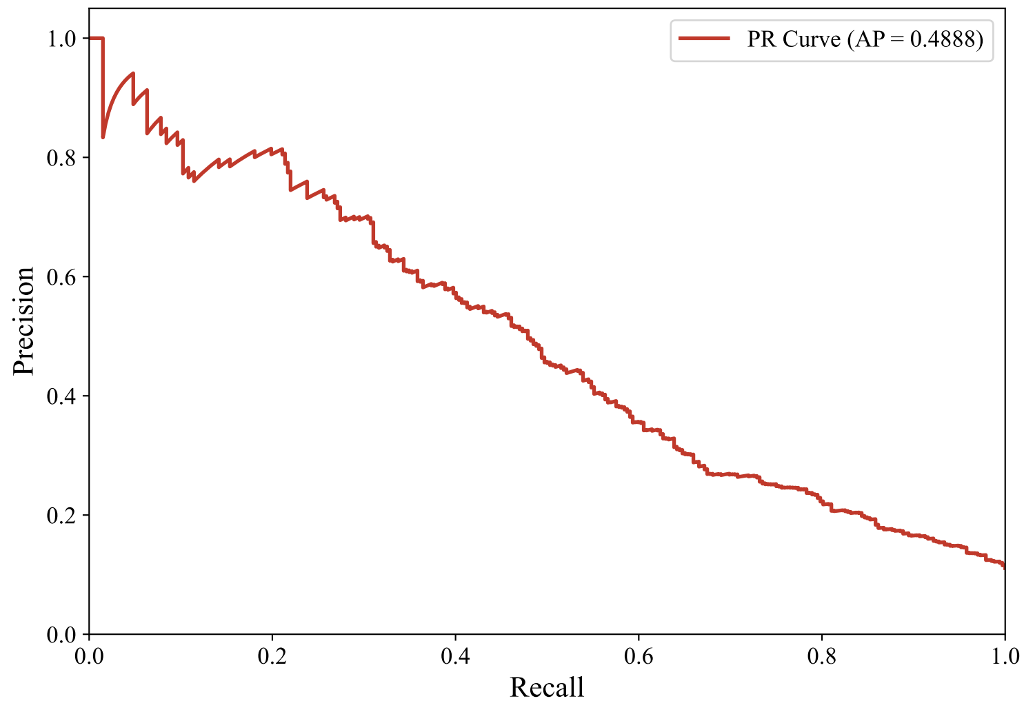
Precision-Recall Curve — GERMAN_MANUAL (xlm-roberta-base, LightGBM)
