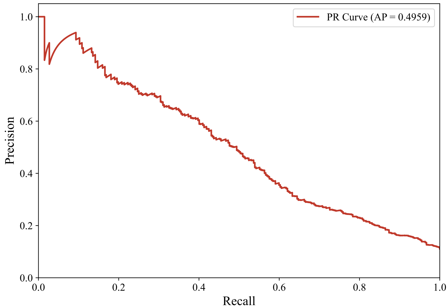
Precision-Recall Curve — GERMAN_MANUAL (xlm-roberta-base, XGBoost)
