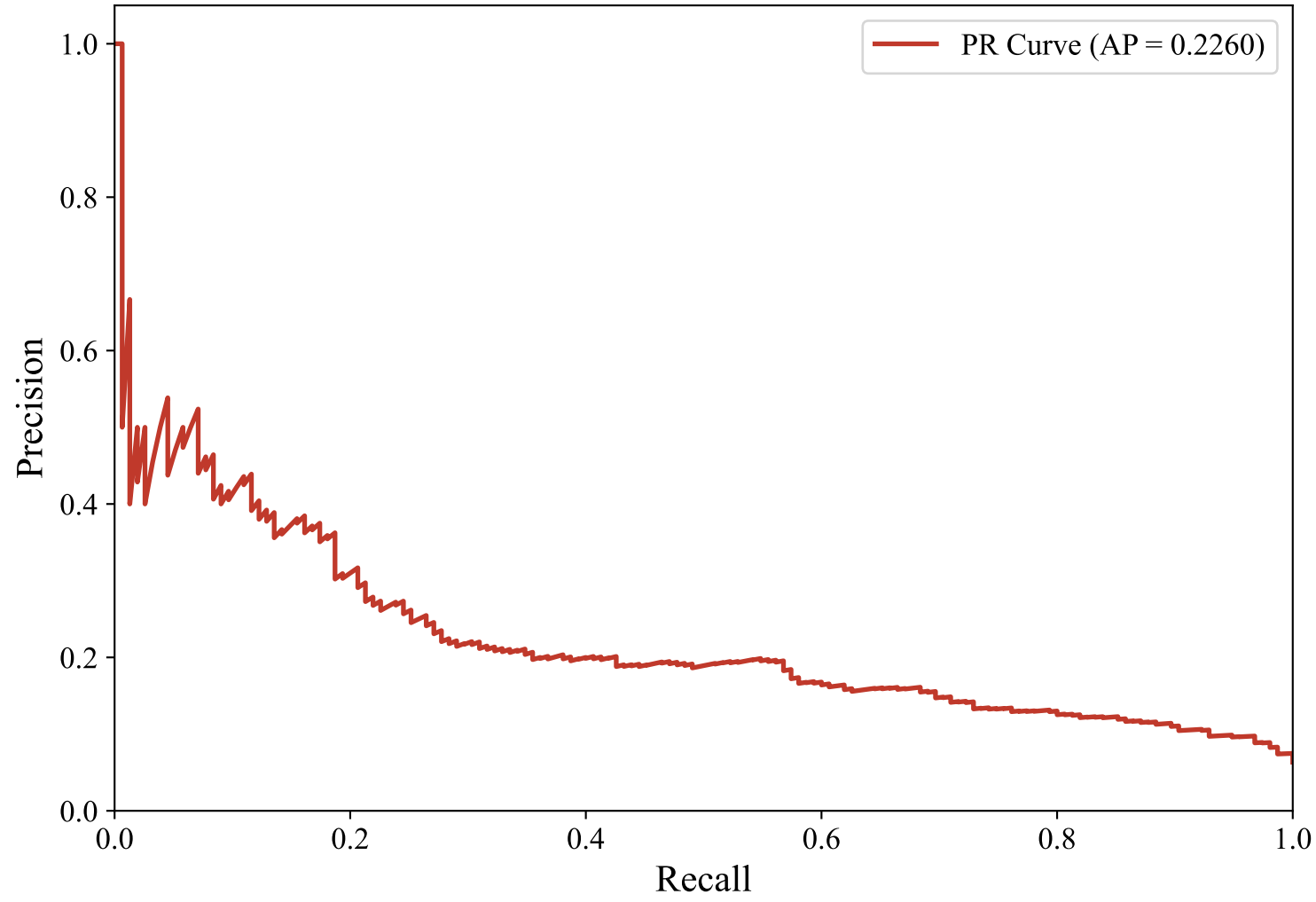
Precision-Recall Curve — SWEDISH_MANUAL (efederici/e5-base-multilingual-4096, LightGBM)
