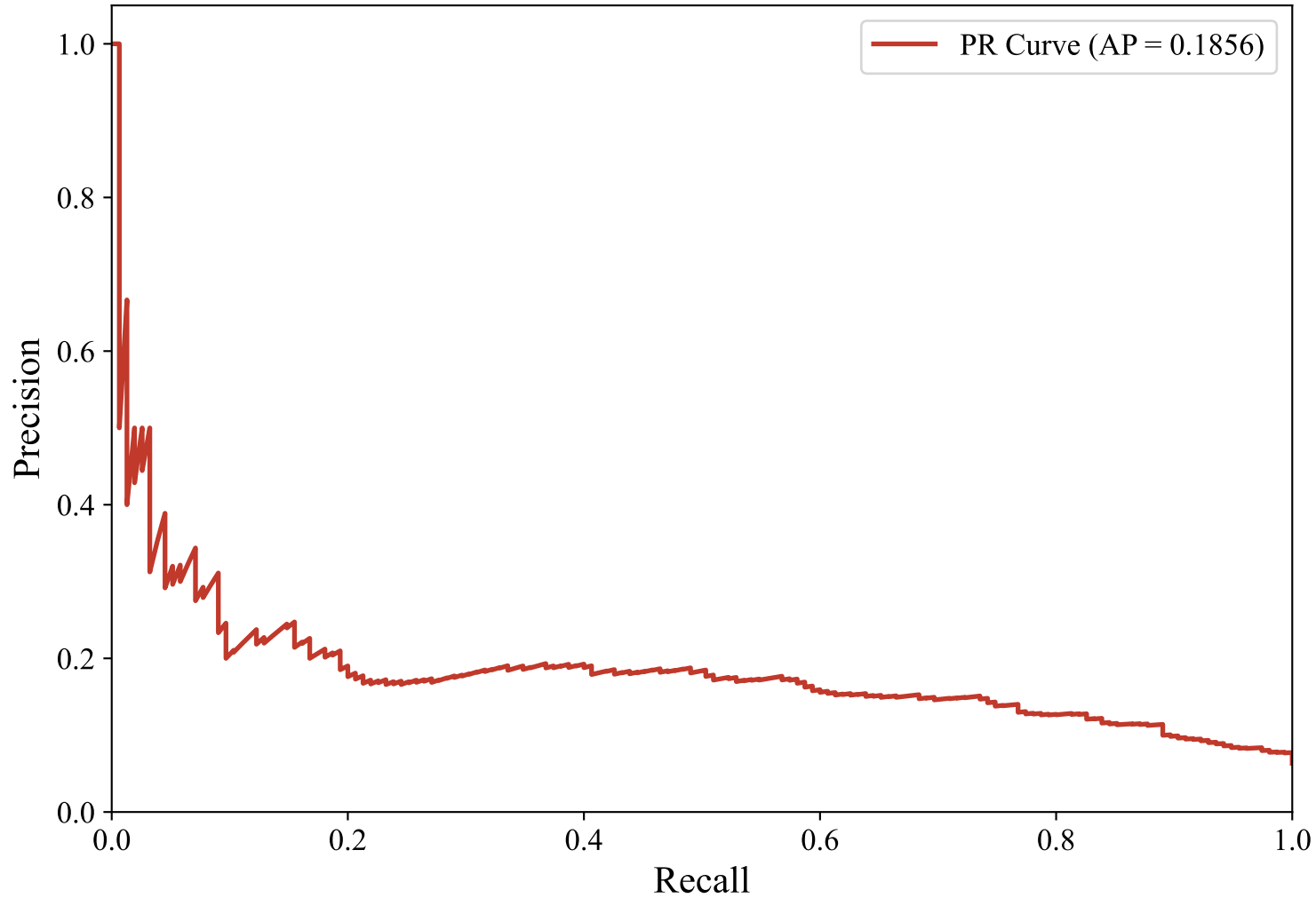
Precision-Recall Curve — SWEDISH_MANUAL (efederici/e5-base-multilingual-4096, Random_Forest)
