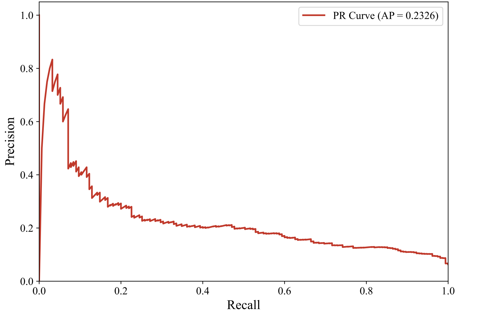
Precision-Recall Curve — SWEDISH_MANUAL (efederici/e5-base-multilingual-4096, XGBoost_Optimized)
