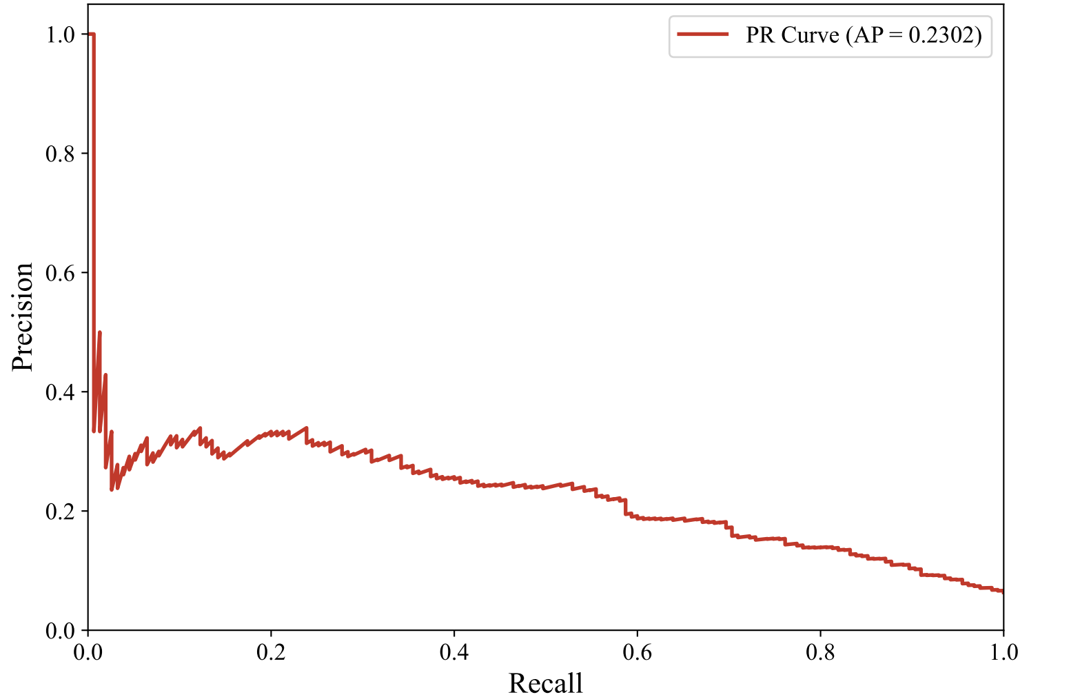
Precision-Recall Curve — SWEDISH_MANUAL (intfloat/multilingual-e5-large-instruct, LightGBM)
