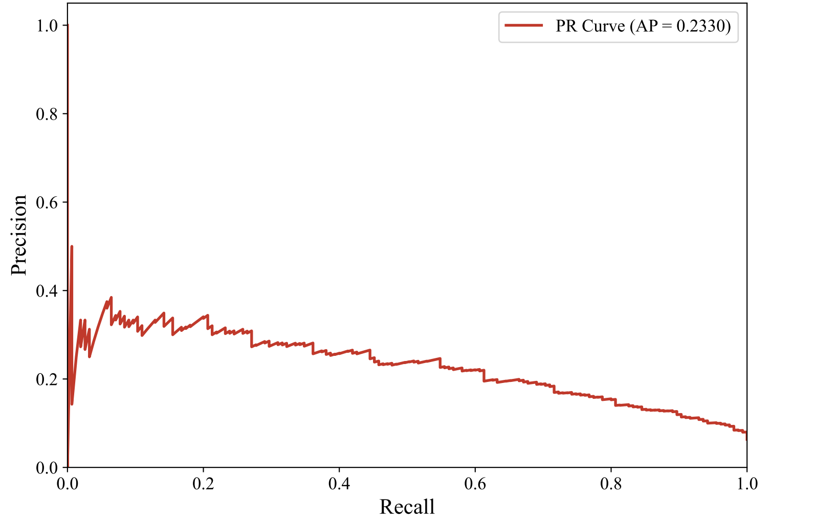
Precision-Recall Curve — SWEDISH_MANUAL (intfloat/multilingual-e5-large-instruct, Voting_Ensemble)
