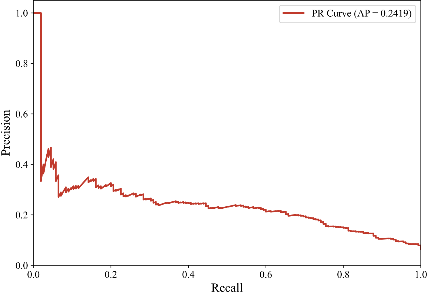
Precision-Recall Curve — SWEDISH_MANUAL (intfloat/multilingual-e5-large-instruct, XGBoost_Optimized)
