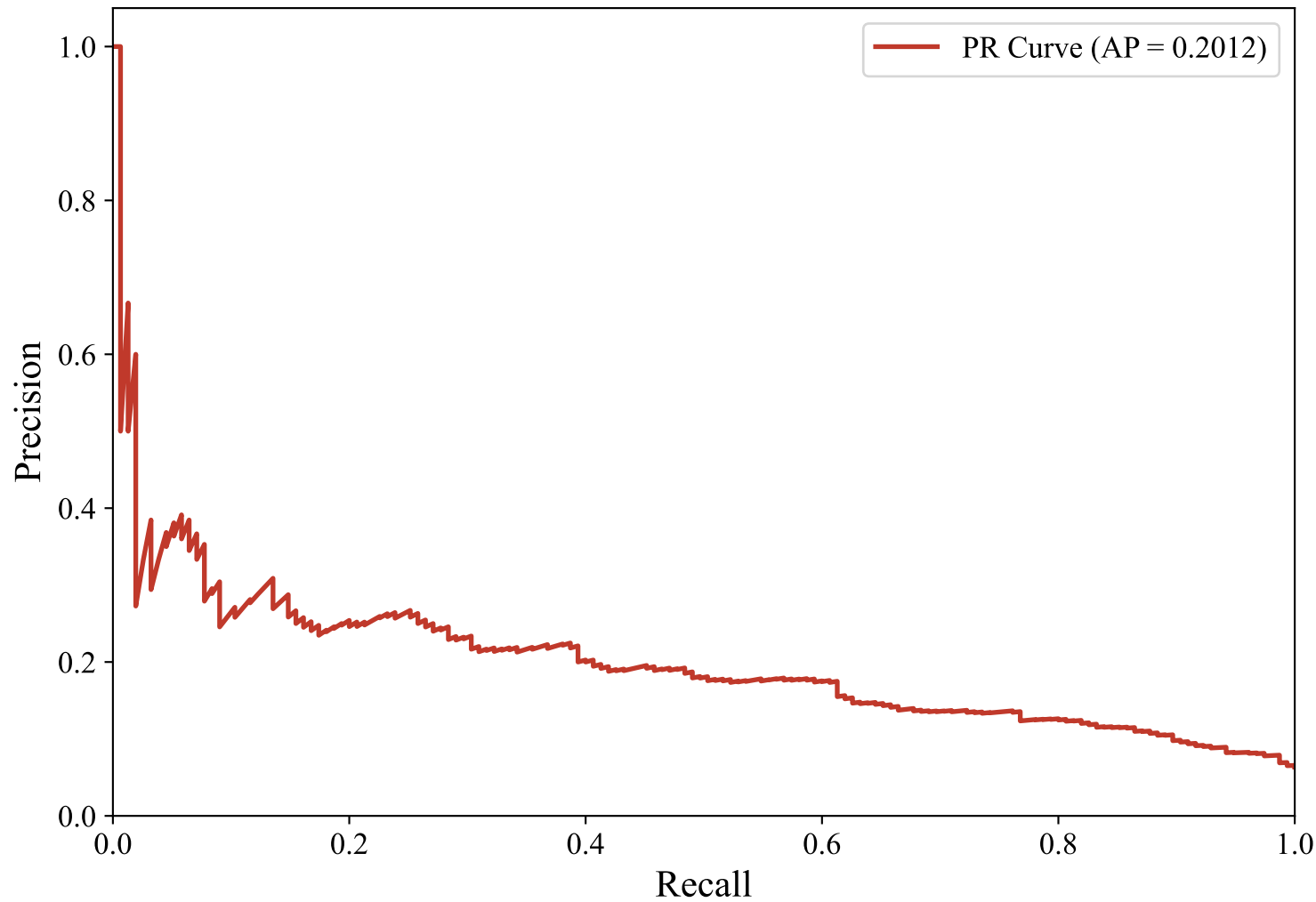
Precision-Recall Curve — SWEDISH_MANUAL (paraphrase-multilingual-MiniLM-L12-v2, LightGBM_Optimized)
