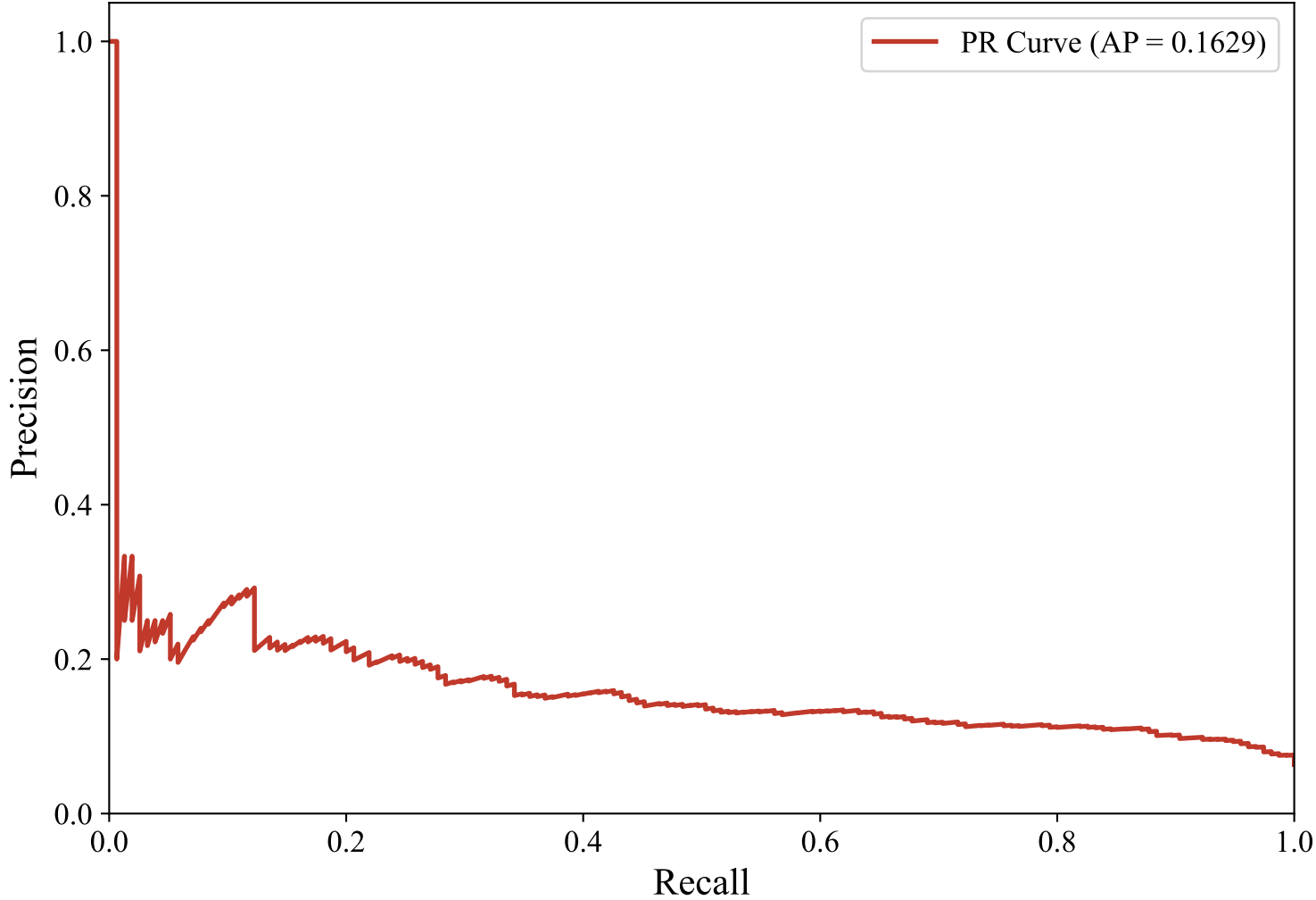
Precision-Recall Curve — SWEDISH_MANUAL (paraphrase-multilingual-MiniLM-L12-v2, Random_Forest)
