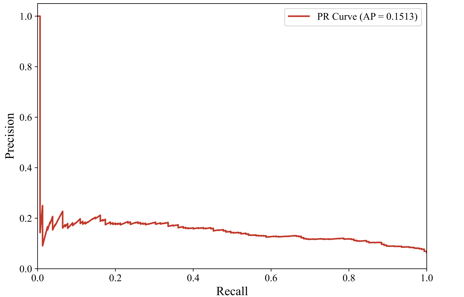
Precision-Recall Curve — SWEDISH_MANUAL (paraphrase-multilingual-mpnet-base-v2, Random_Forest)
