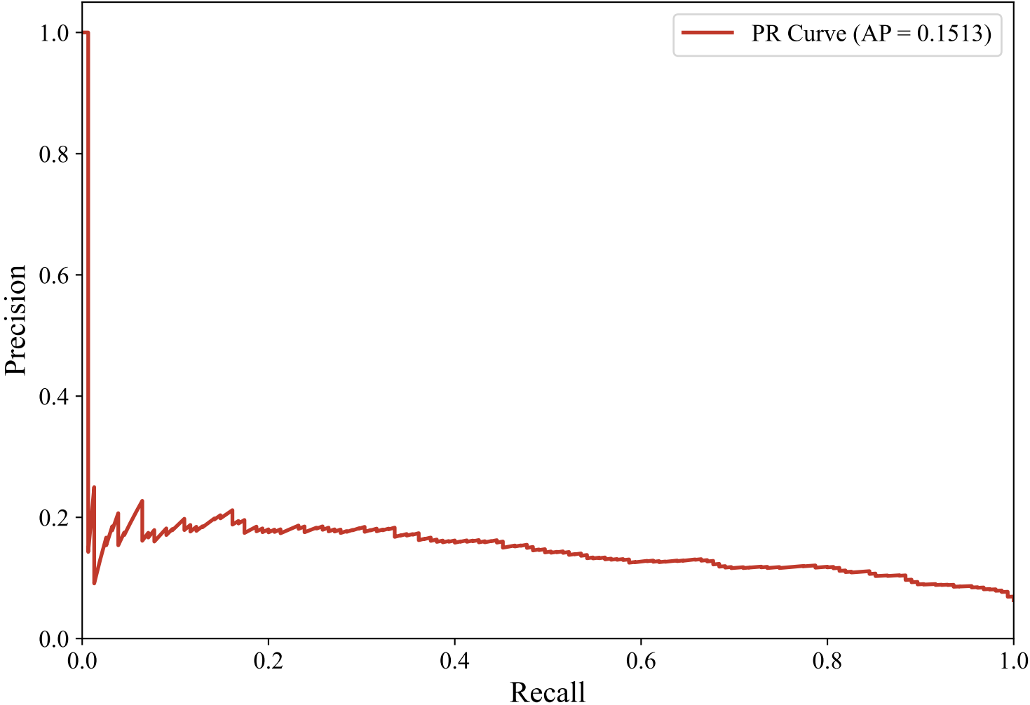
Precision-Recall Curve — SWEDISH_MANUAL (paraphrase-multilingual-mpnet-base-v2, Random_Forest_Optimized)
