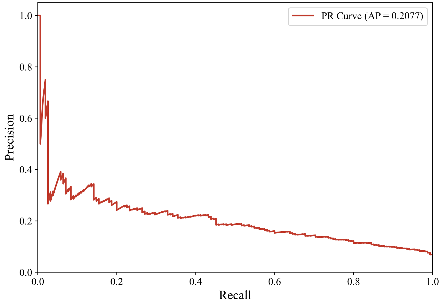
Precision-Recall Curve — SWEDISH_MANUAL (paraphrase-multilingual-mpnet-base-v2, Voting_Ensemble)
