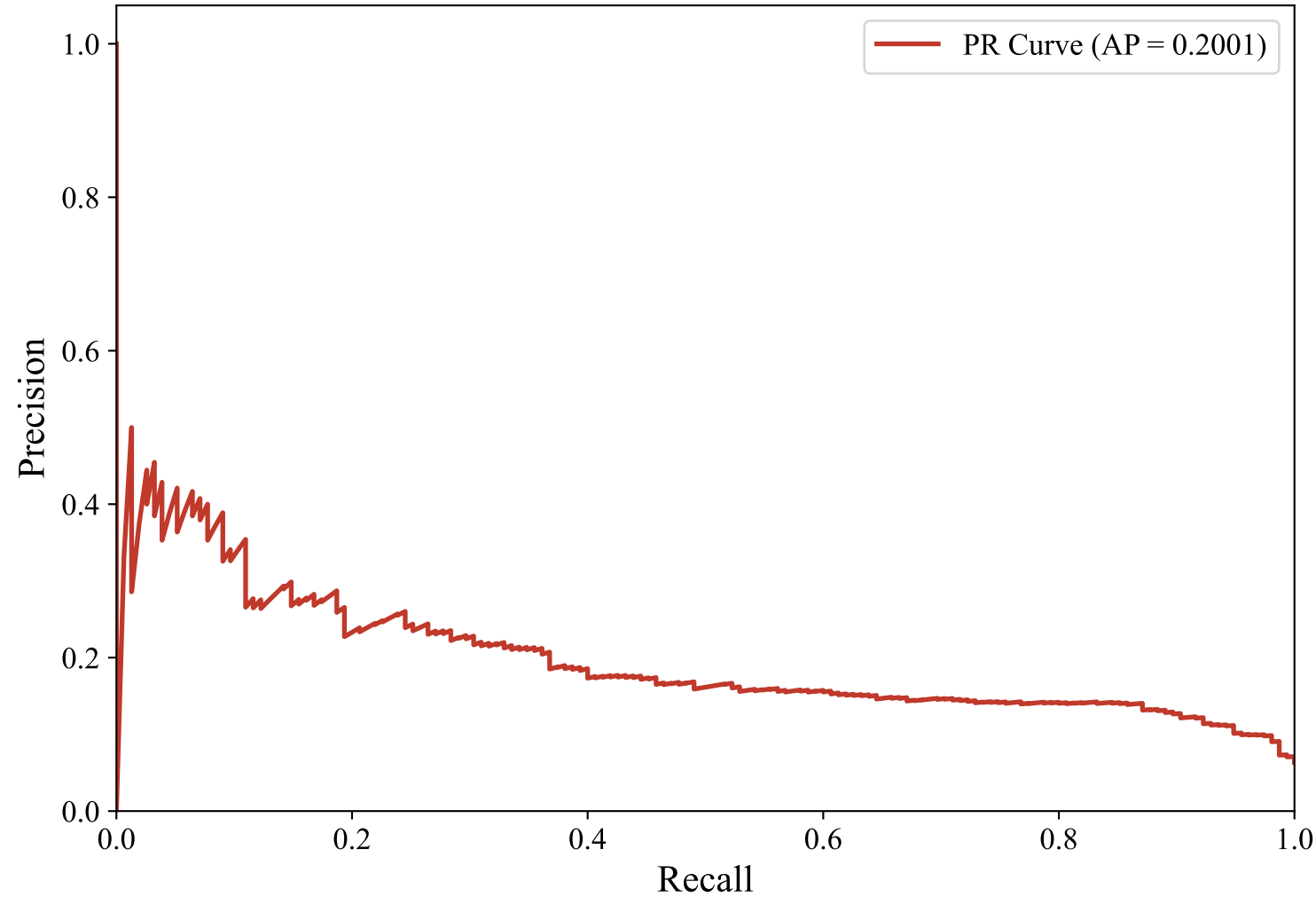
Precision-Recall Curve — SWEDISH_MANUAL (upskyy/bge-m3-korean, Random_Forest)
