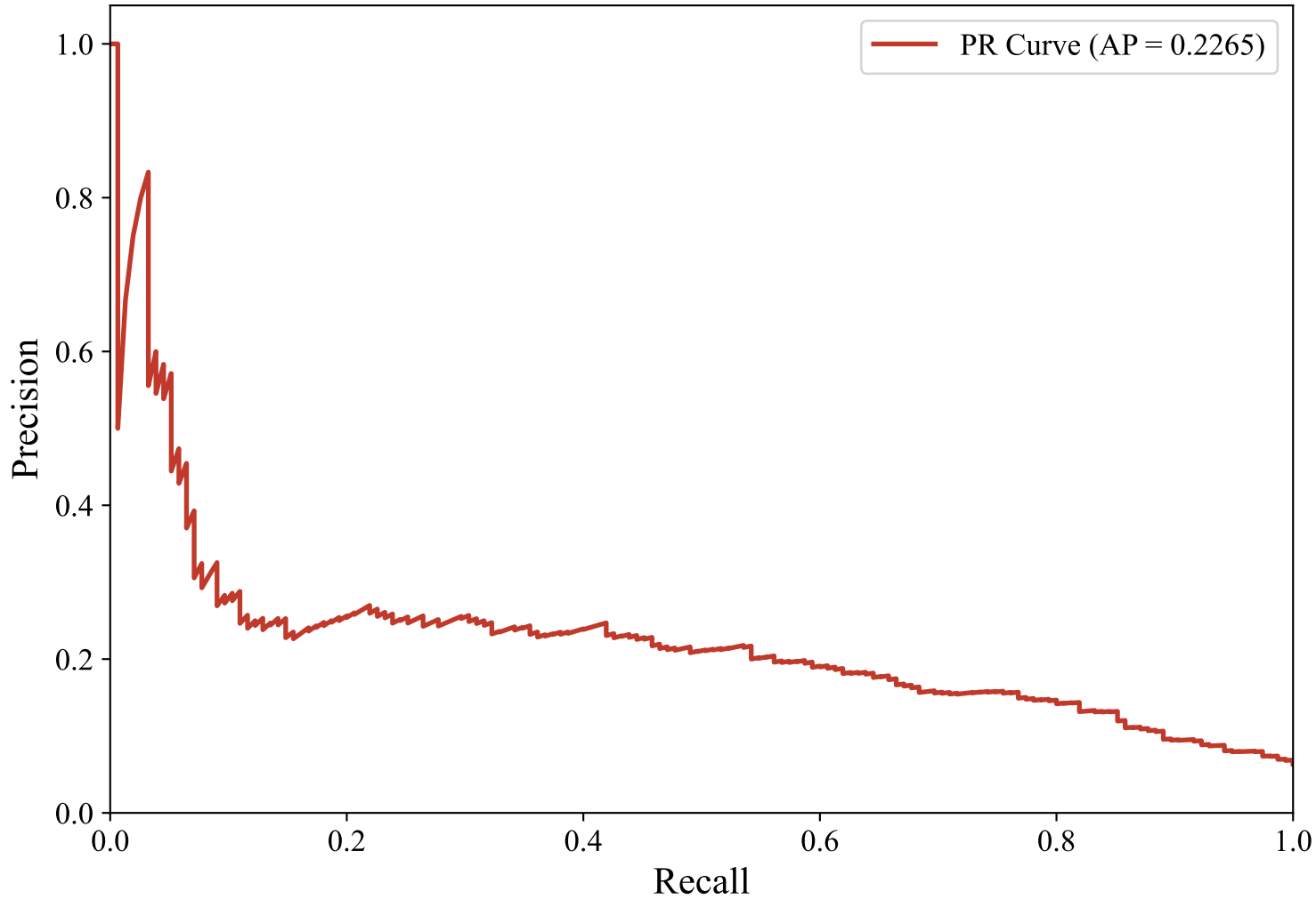
Precision-Recall Curve — SWEDISH_MANUAL (upskyy/bge-m3-korean, XGBoost)
