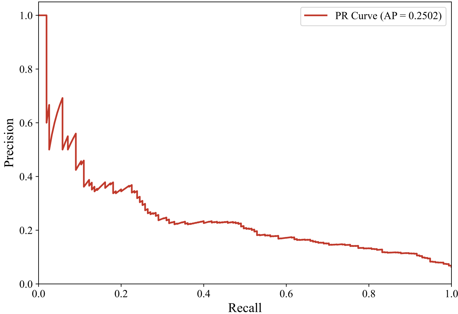
Precision-Recall Curve — SWEDISH_MANUAL (xlm-roberta-base, LightGBM)
