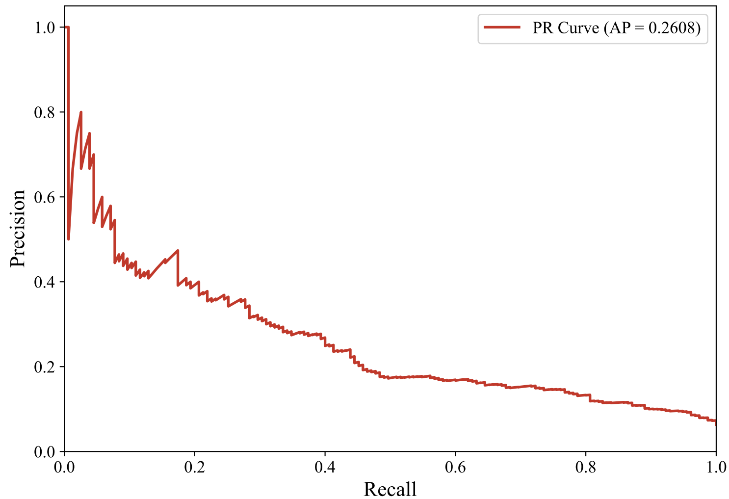
Precision-Recall Curve — SWEDISH_MANUAL (xlm-roberta-base, XGBoost_Optimized)
