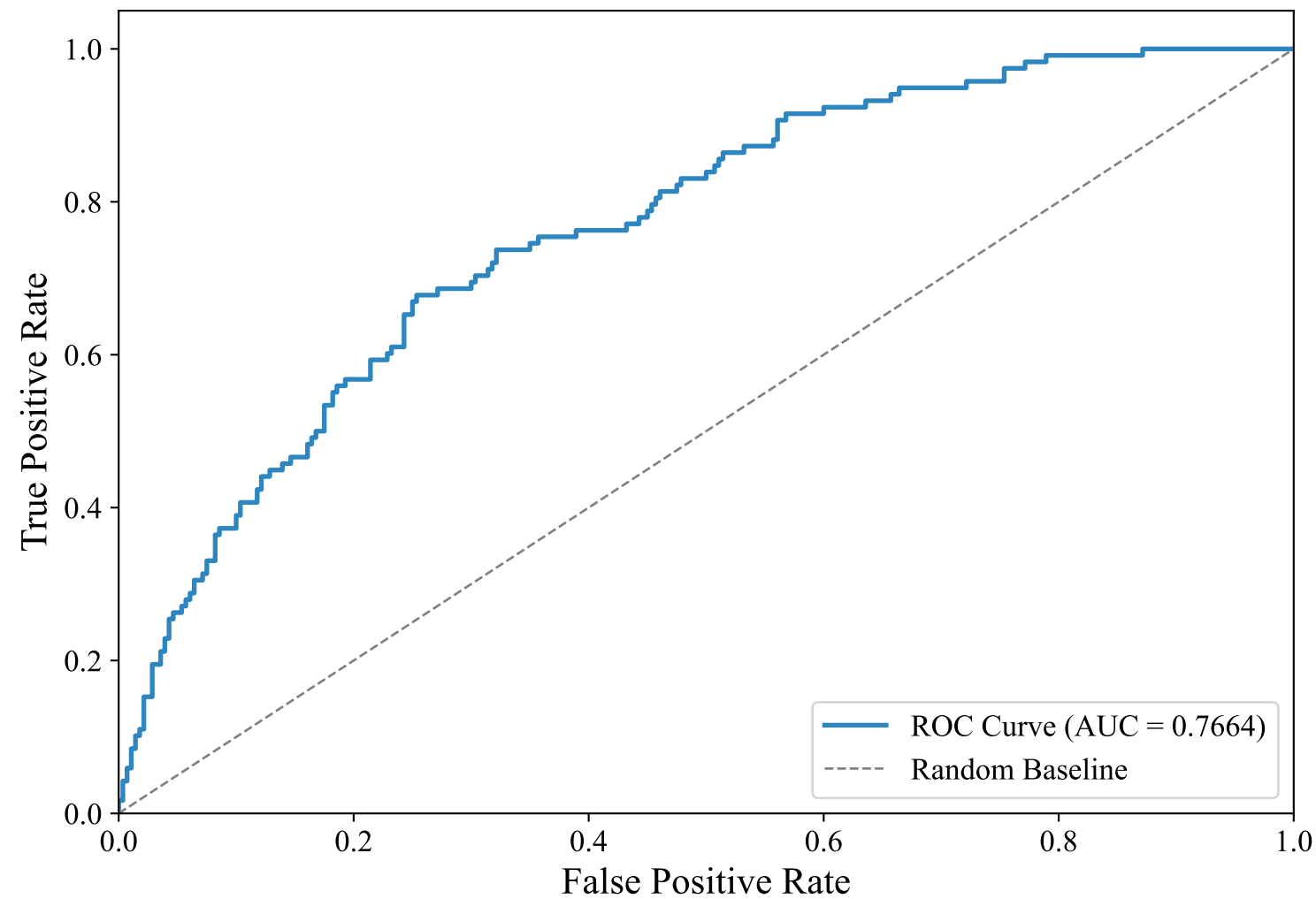
ROC Curve — DUTCH_MANUAL (bert-base-multilingual-uncased, LightGBM_Optimized)
