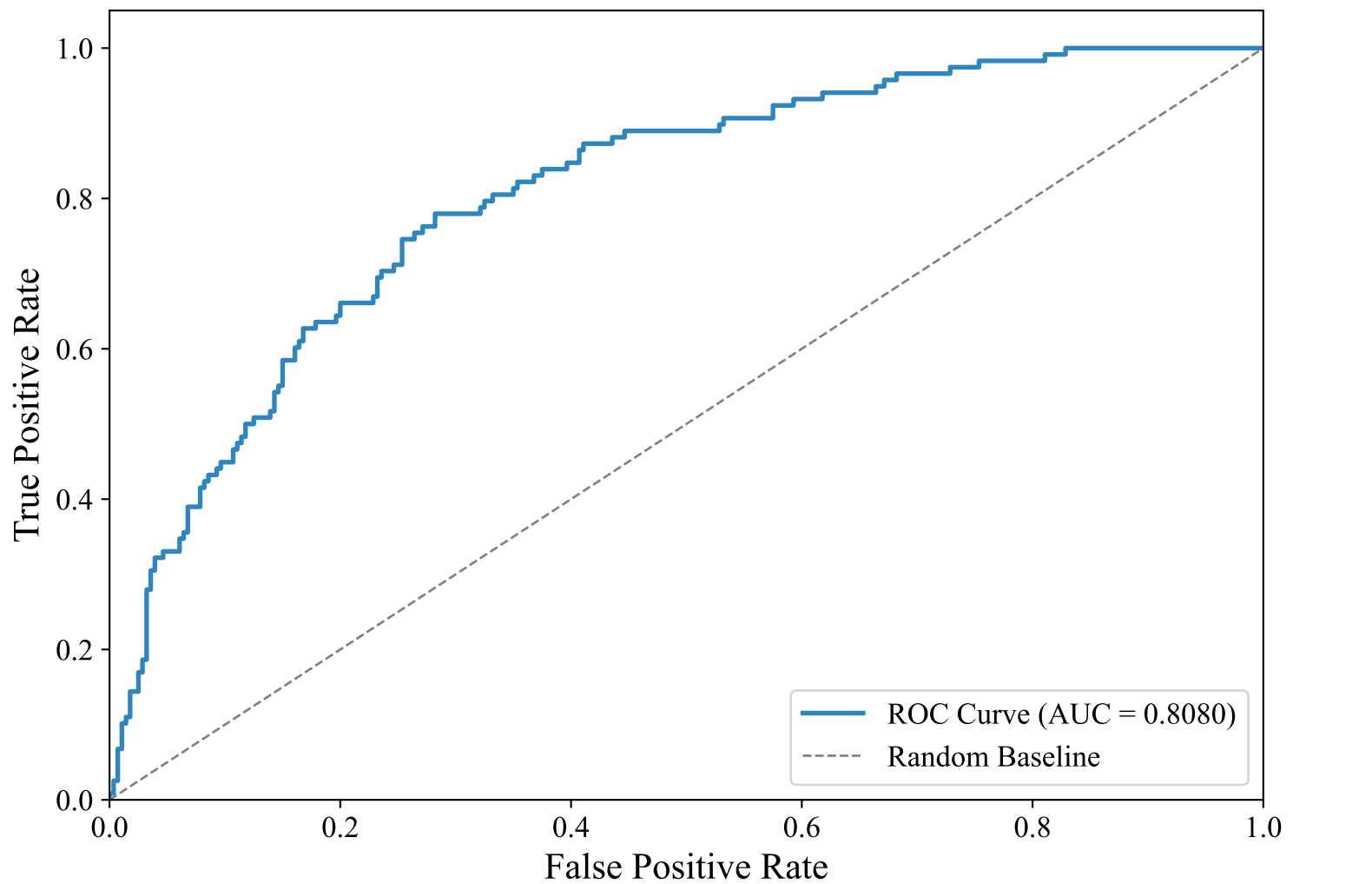
ROC Curve — DUTCH_MANUAL (efederici/e5-base-multilingual-4096, LightGBM_Optimized)
