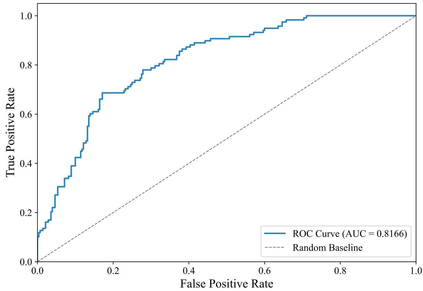
ROC Curve — DUTCH_MANUAL (efederici/e5-base-multilingual-4096, Voting_Ensemble)
