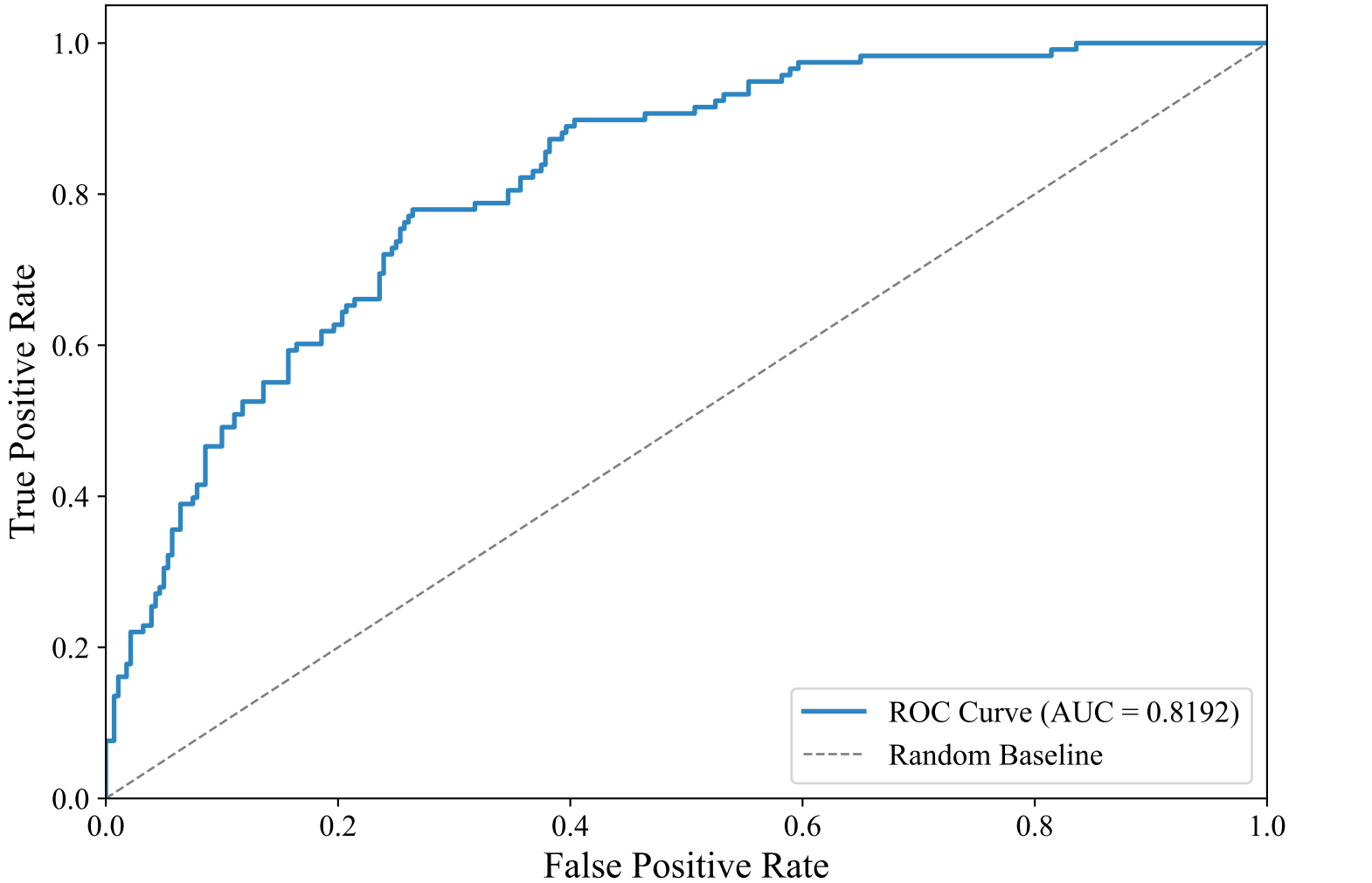
ROC Curve — DUTCH_MANUAL (efederici/e5-base-multilingual-4096, XGBoost)
