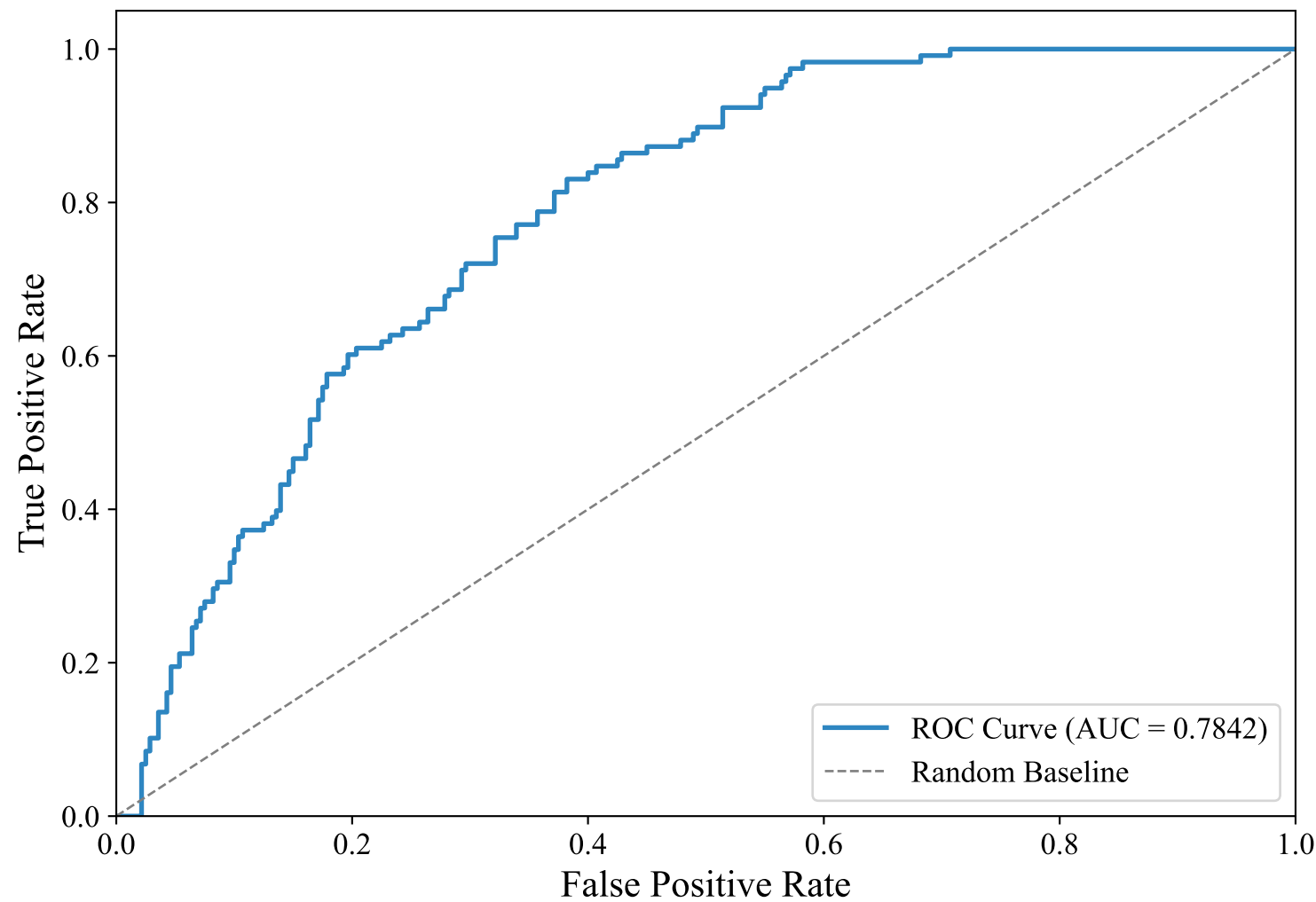
ROC Curve — DUTCH_MANUAL (intfloat/multilingual-e5-large-instruct, Random_Forest)
