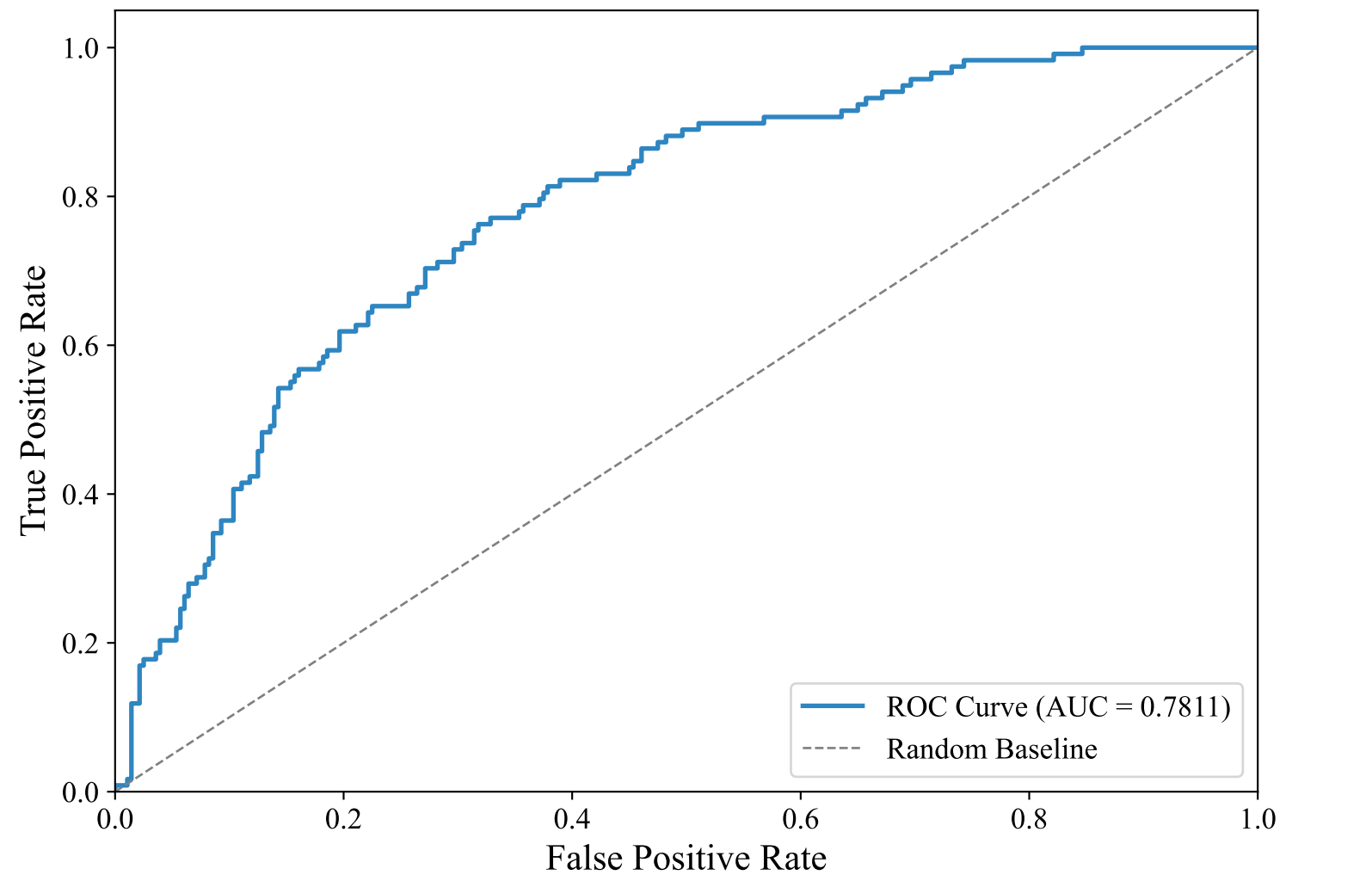
ROC Curve — DUTCH_MANUAL (paraphrase-multilingual-MiniLM-L12-v2, LightGBM_Optimized)
