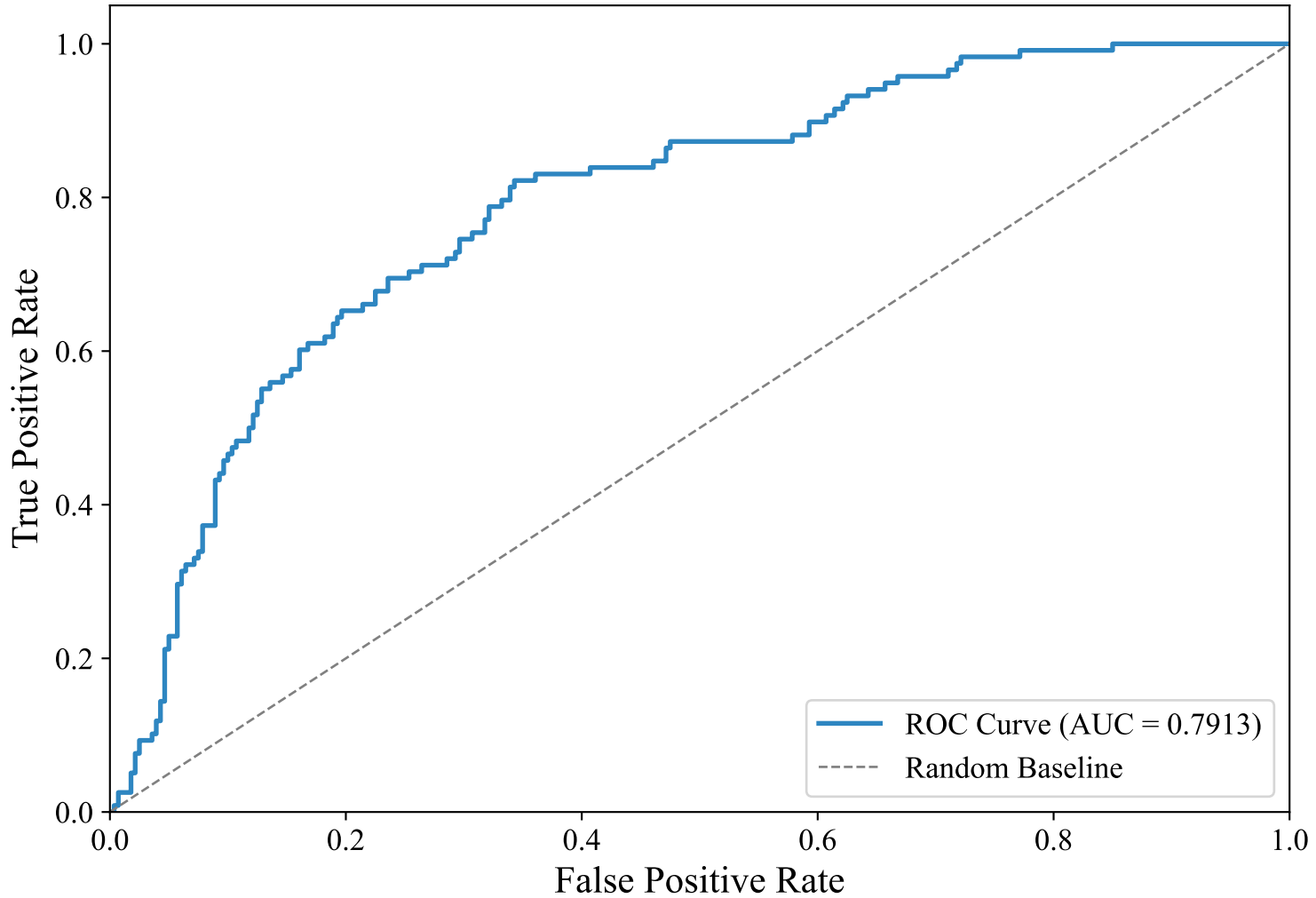
ROC Curve — DUTCH_MANUAL (paraphrase-multilingual-MiniLM-L12-v2, XGBoost)
