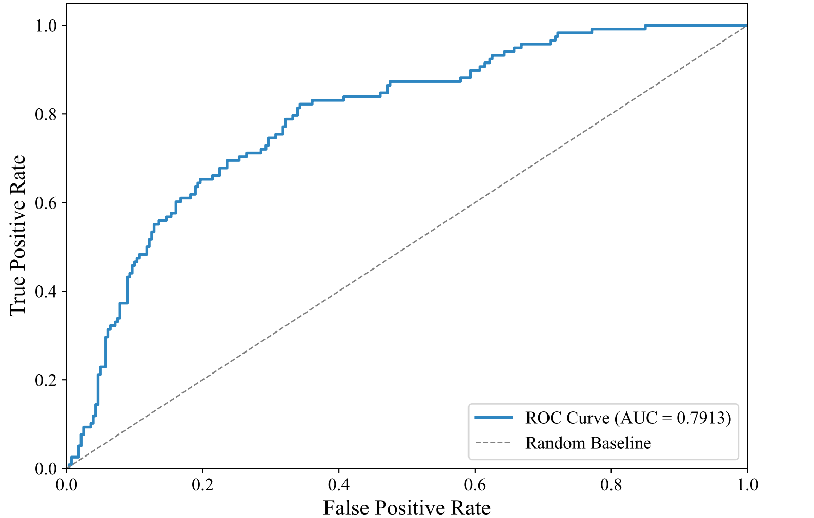
ROC Curve — DUTCH_MANUAL (paraphrase-multilingual-MiniLM-L12-v2, XGBoost_Optimized)
