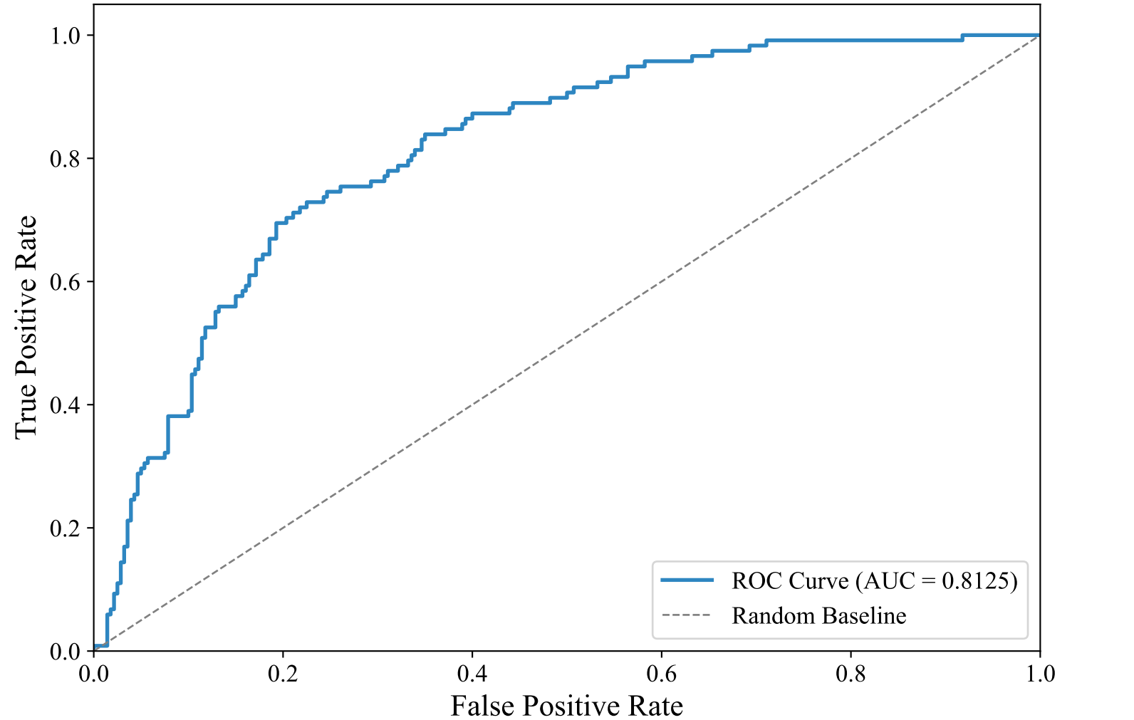
ROC Curve — DUTCH_MANUAL (paraphrase-multilingual-mpnet-base-v2, LightGBM_Optimized)
