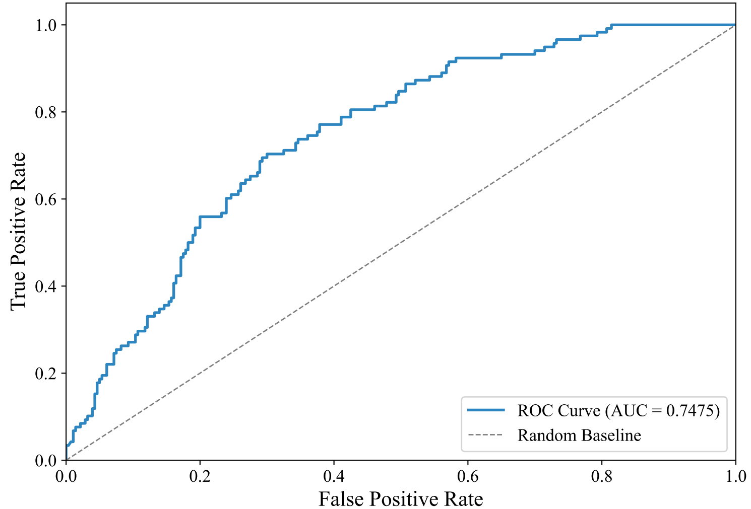
ROC Curve — DUTCH_MANUAL (paraphrase-multilingual-mpnet-base-v2, Random_Forest)
