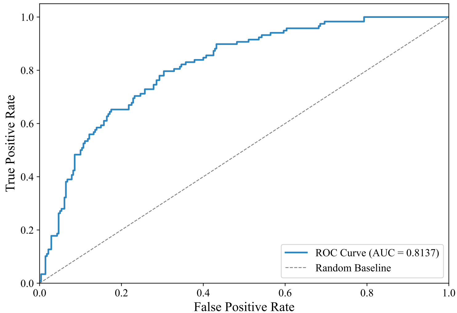
ROC Curve — DUTCH_MANUAL (paraphrase-multilingual-mpnet-base-v2, XGBoost)
