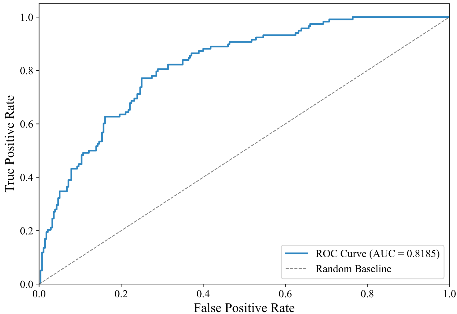
ROC Curve — DUTCH_MANUAL (snowflake-arctic-embed-l-v2.0, LightGBM)
