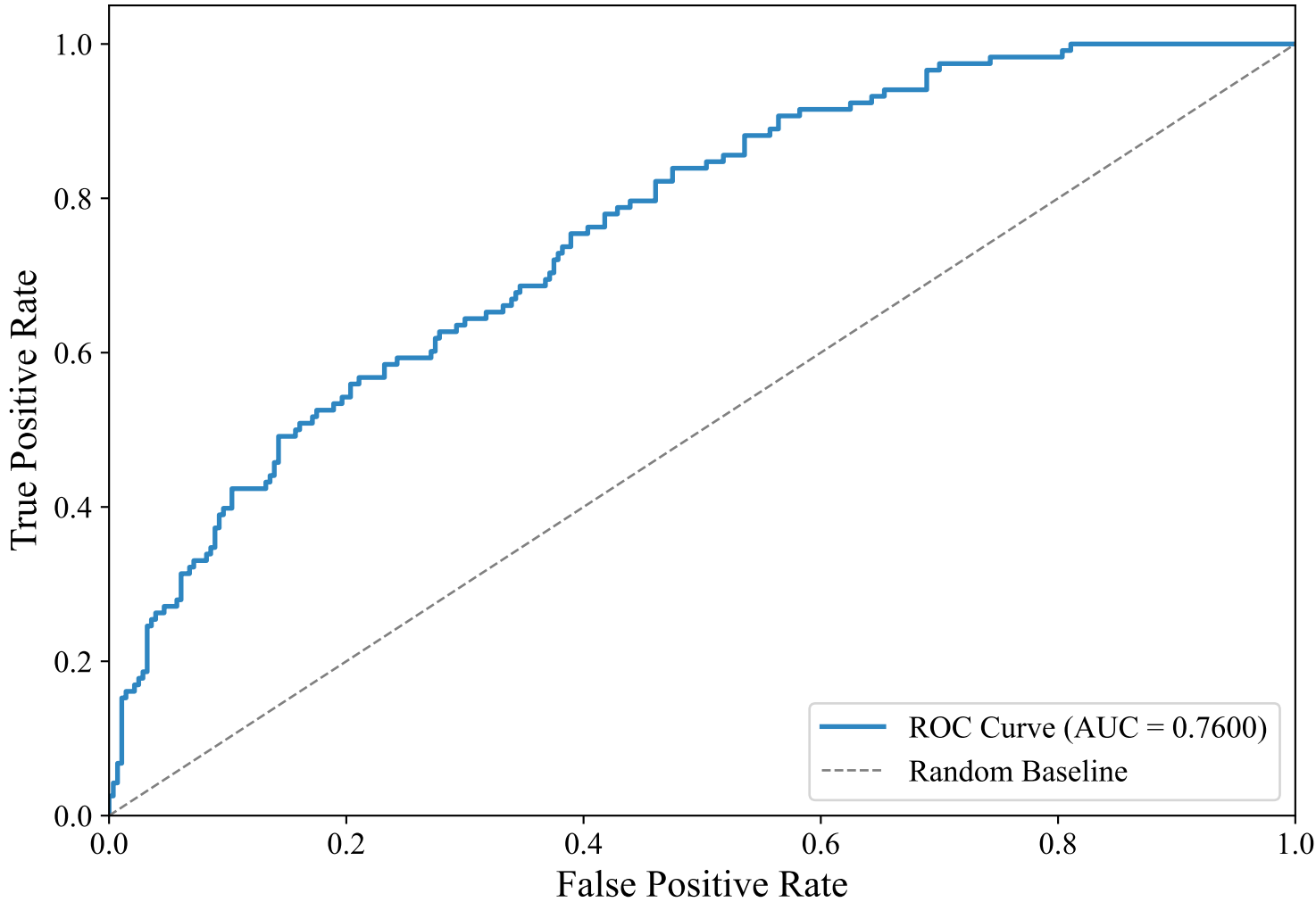
ROC Curve — DUTCH_MANUAL (upskyy/bge-m3-korean, Random_Forest)
