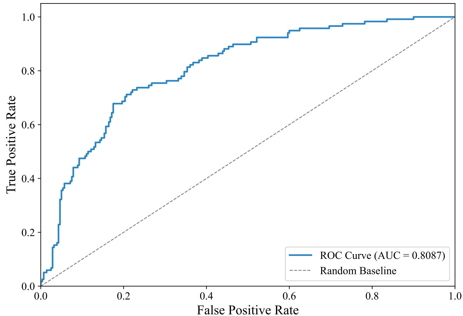
ROC Curve — DUTCH_MANUAL (upskyy/bge-m3-korean, XGBoost)
