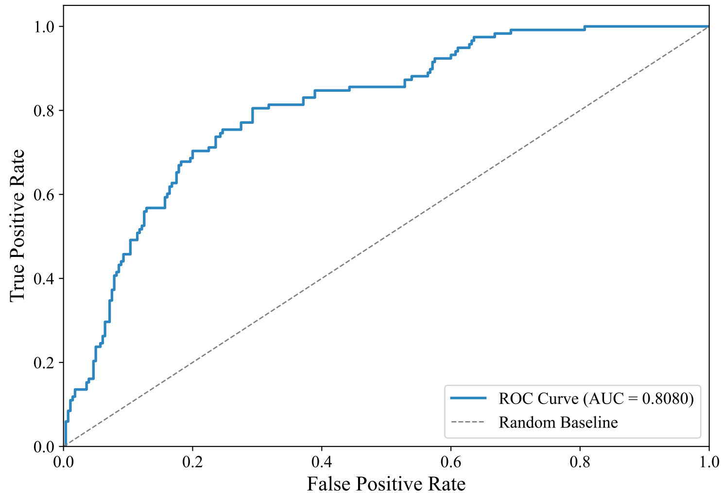
ROC Curve — DUTCH_MANUAL (xlm-roberta-base, Voting_Ensemble)
