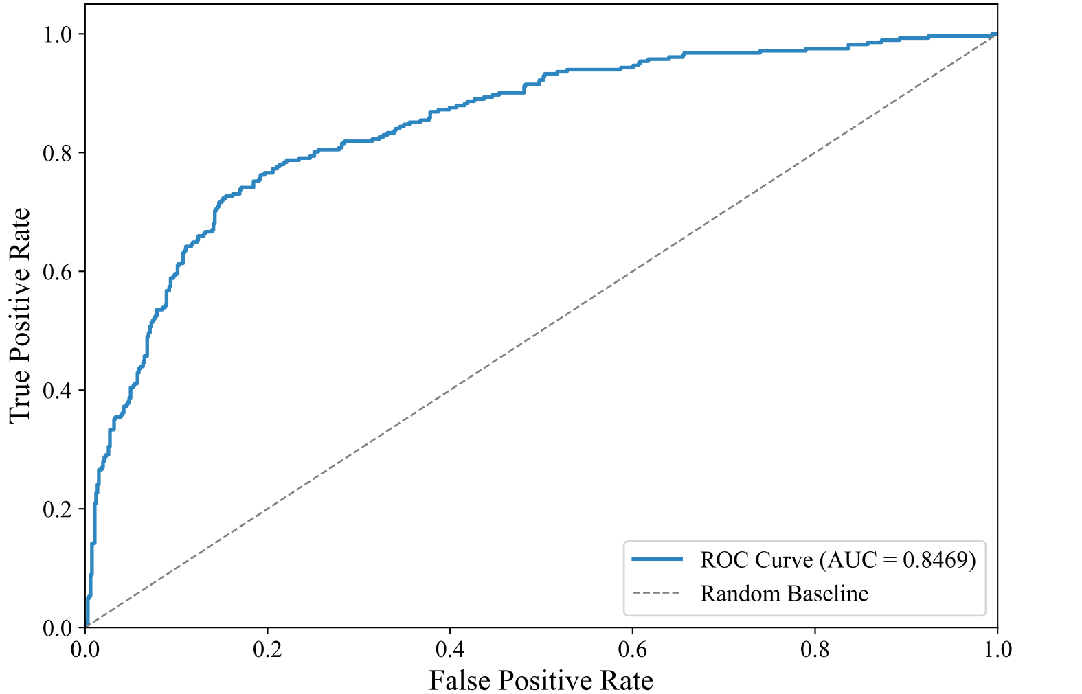
ROC Curve — ENGLISH_MANUAL (bert-base-multilingual-uncased, LightGBM)
