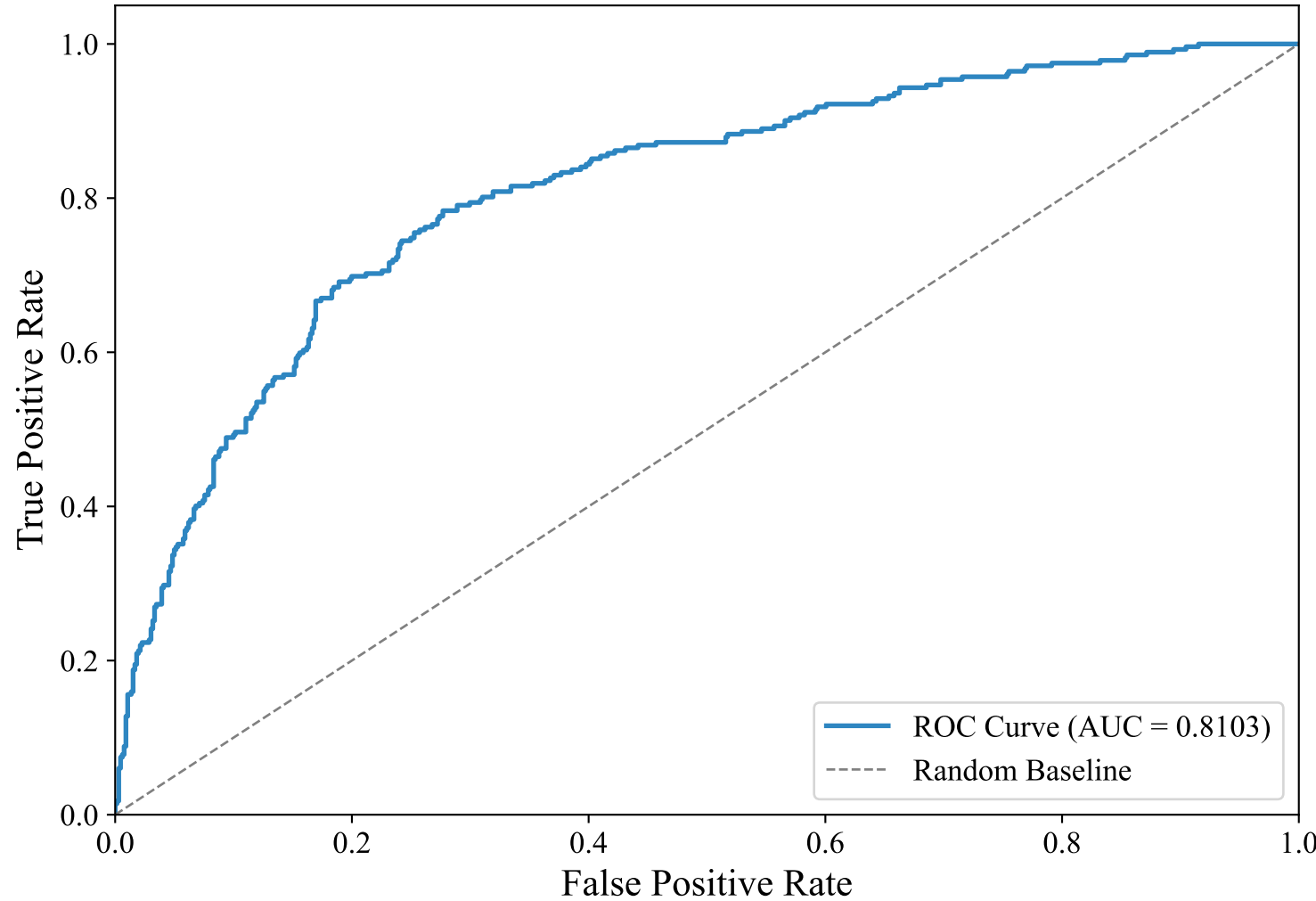
ROC Curve — ENGLISH_MANUAL (efederici/e5-base-multilingual-4096, Random_Forest_Optimized)
