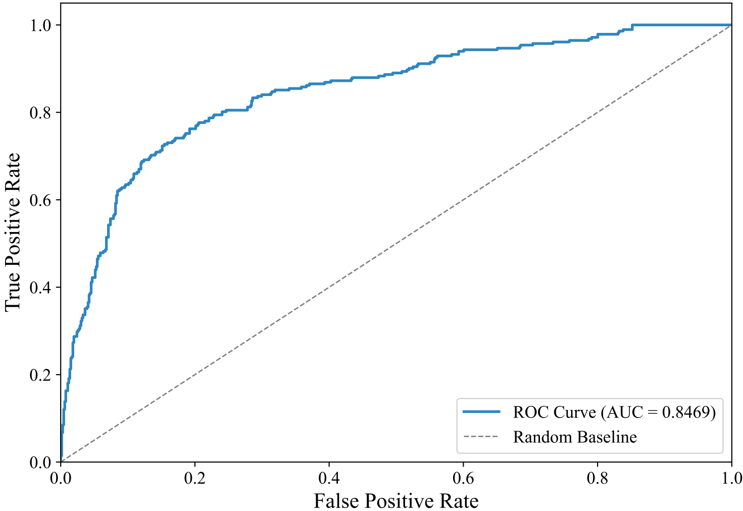
ROC Curve — ENGLISH_MANUAL (efederici/e5-base-multilingual-4096, Voting_Ensemble)
