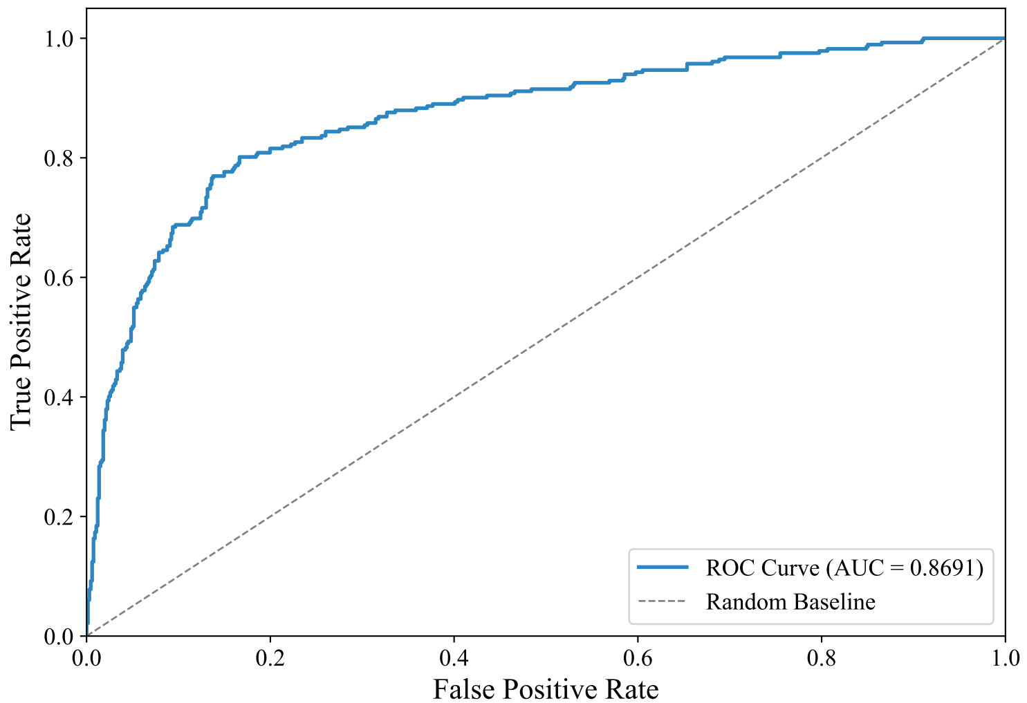
ROC Curve — ENGLISH_MANUAL (intfloat/multilingual-e5-large-instruct, LightGBM)
