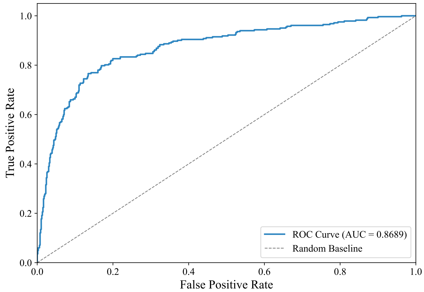
ROC Curve — ENGLISH_MANUAL (intfloat/multilingual-e5-large-instruct, Voting_Ensemble)
