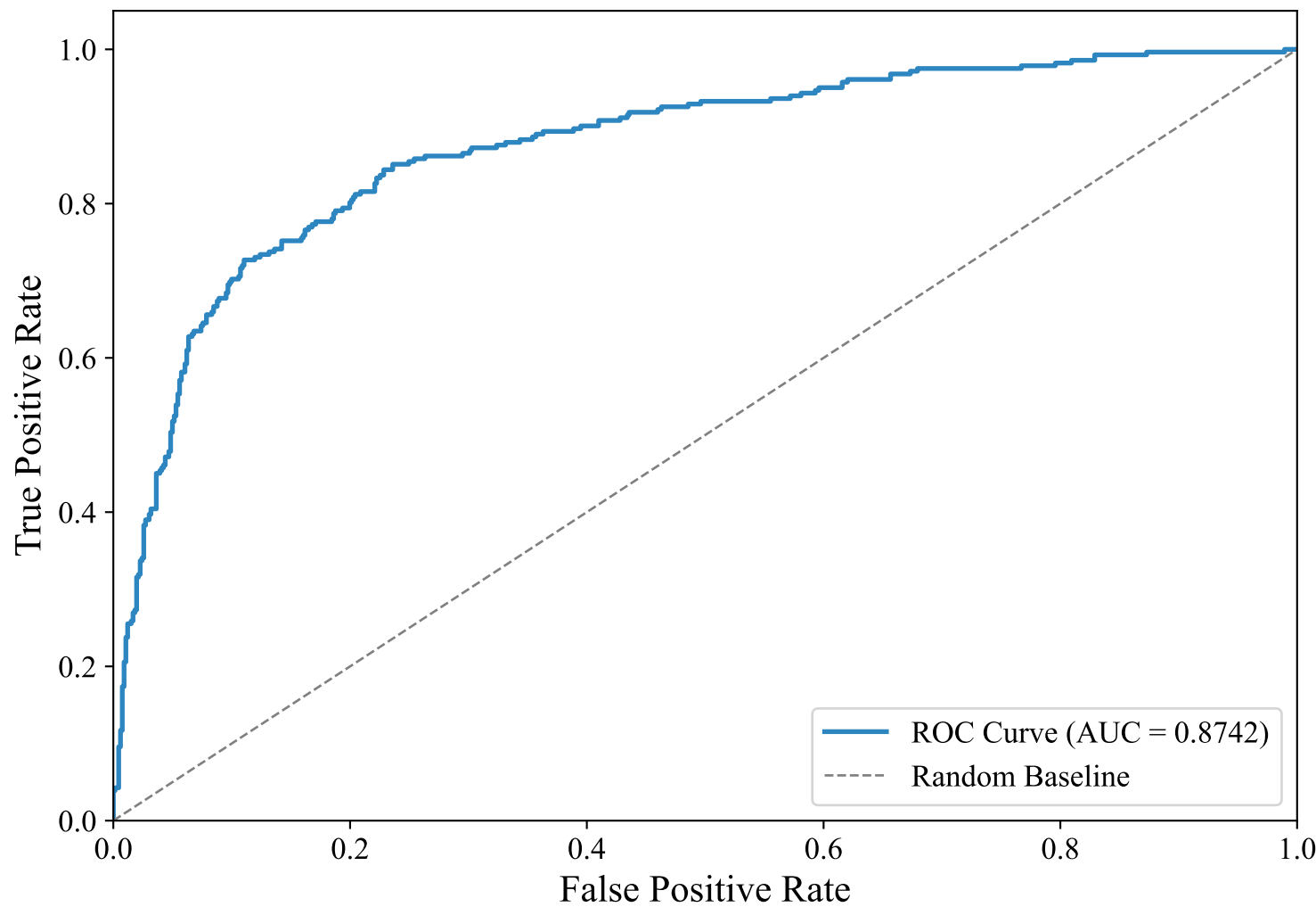
ROC Curve — ENGLISH_MANUAL (intfloat/multilingual-e5-large-instruct, XGBoost_Optimized)
