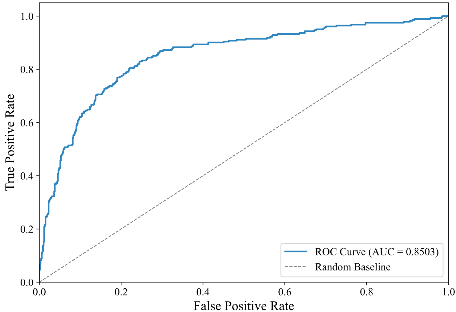
ROC Curve — ENGLISH_MANUAL (paraphrase-multilingual-MiniLM-L12-v2, LightGBM_Optimized)
