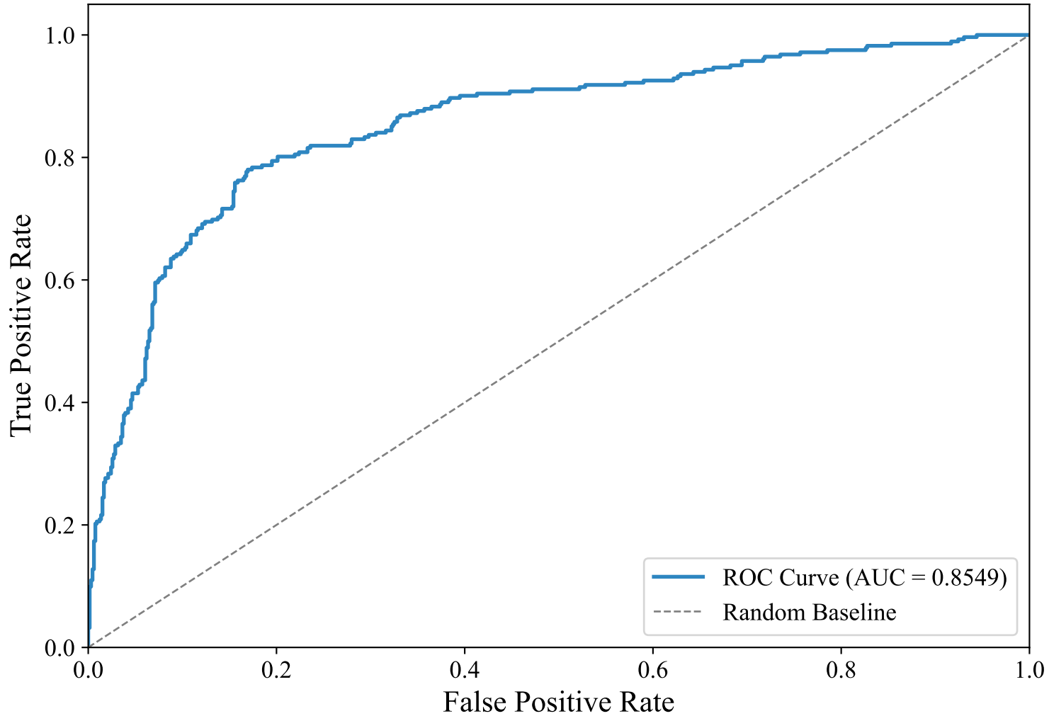
ROC Curve — ENGLISH_MANUAL (paraphrase-multilingual-MiniLM-L12-v2, XGBoost)
