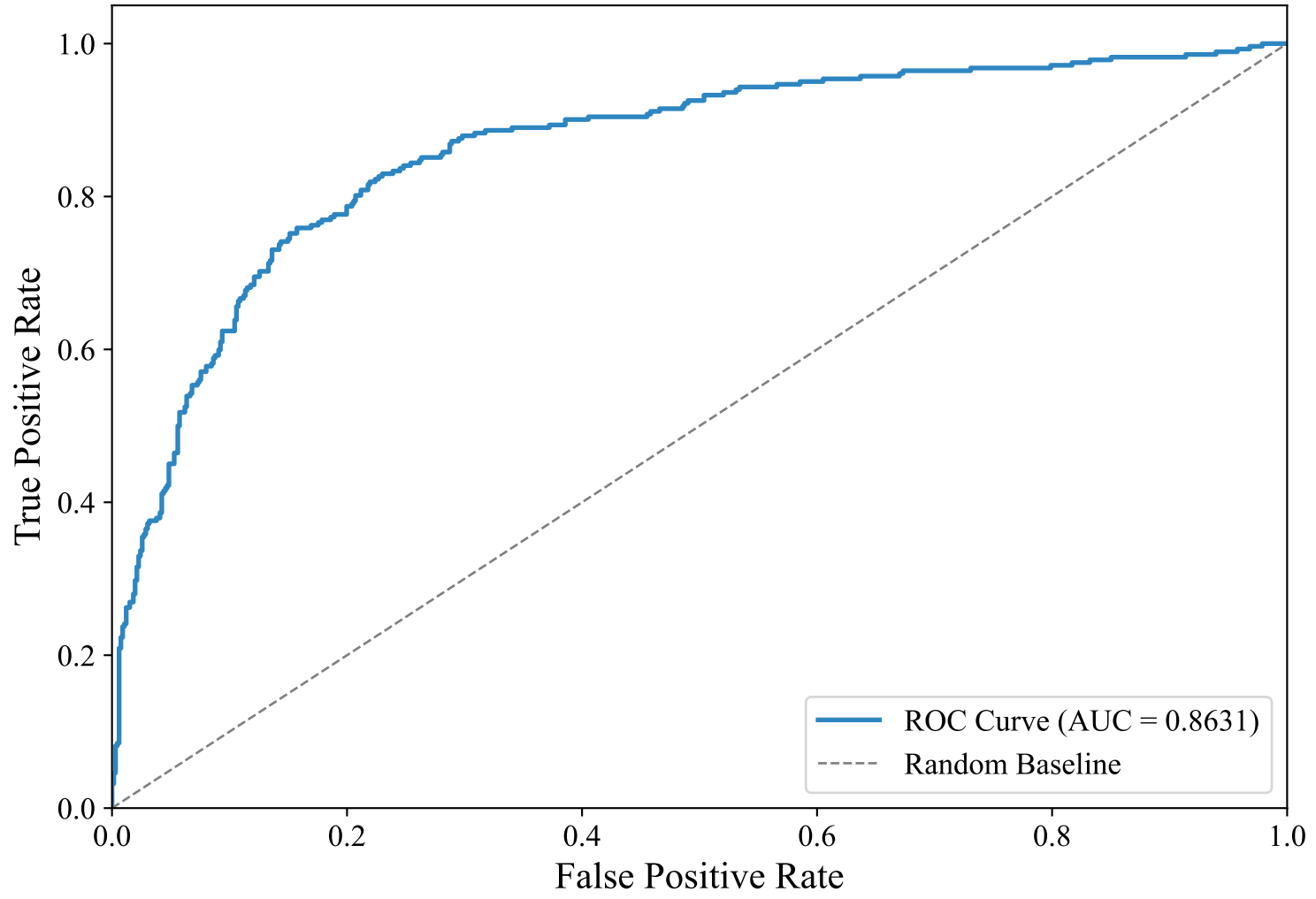
ROC Curve — ENGLISH_MANUAL (snowflake-arctic-embed-l-v2.0, Voting_Ensemble)
