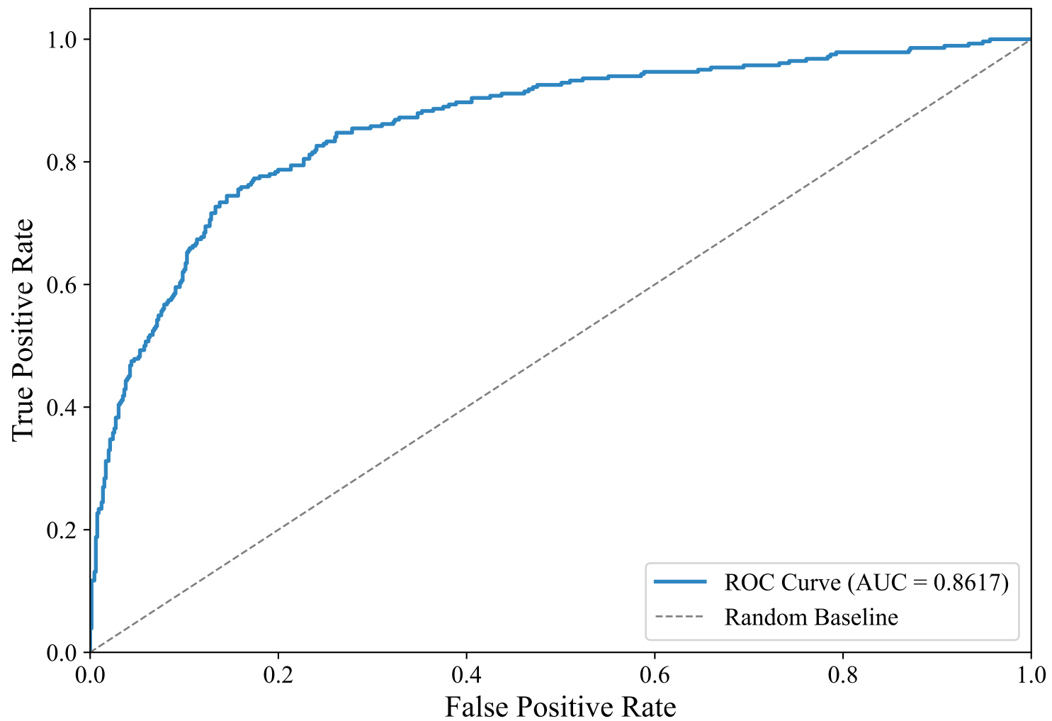
ROC Curve — ENGLISH_MANUAL (snowflake-arctic-embed-l-v2.0, XGBoost_Optimized)
