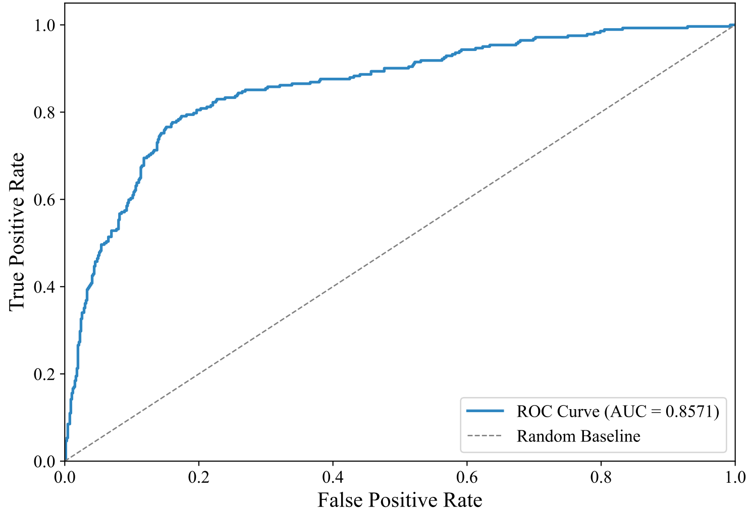
ROC Curve — ENGLISH_MANUAL (upskyy/bge-m3-korean, LightGBM_Optimized)
