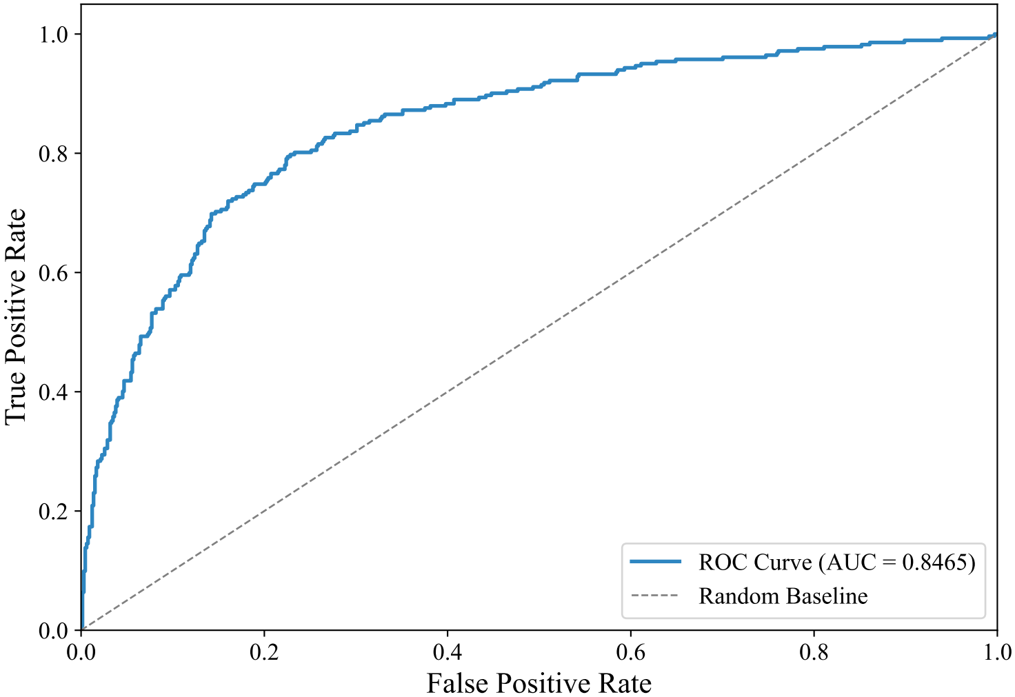
ROC Curve — ENGLISH_MANUAL (xlm-roberta-base, XGBoost_Optimized)
