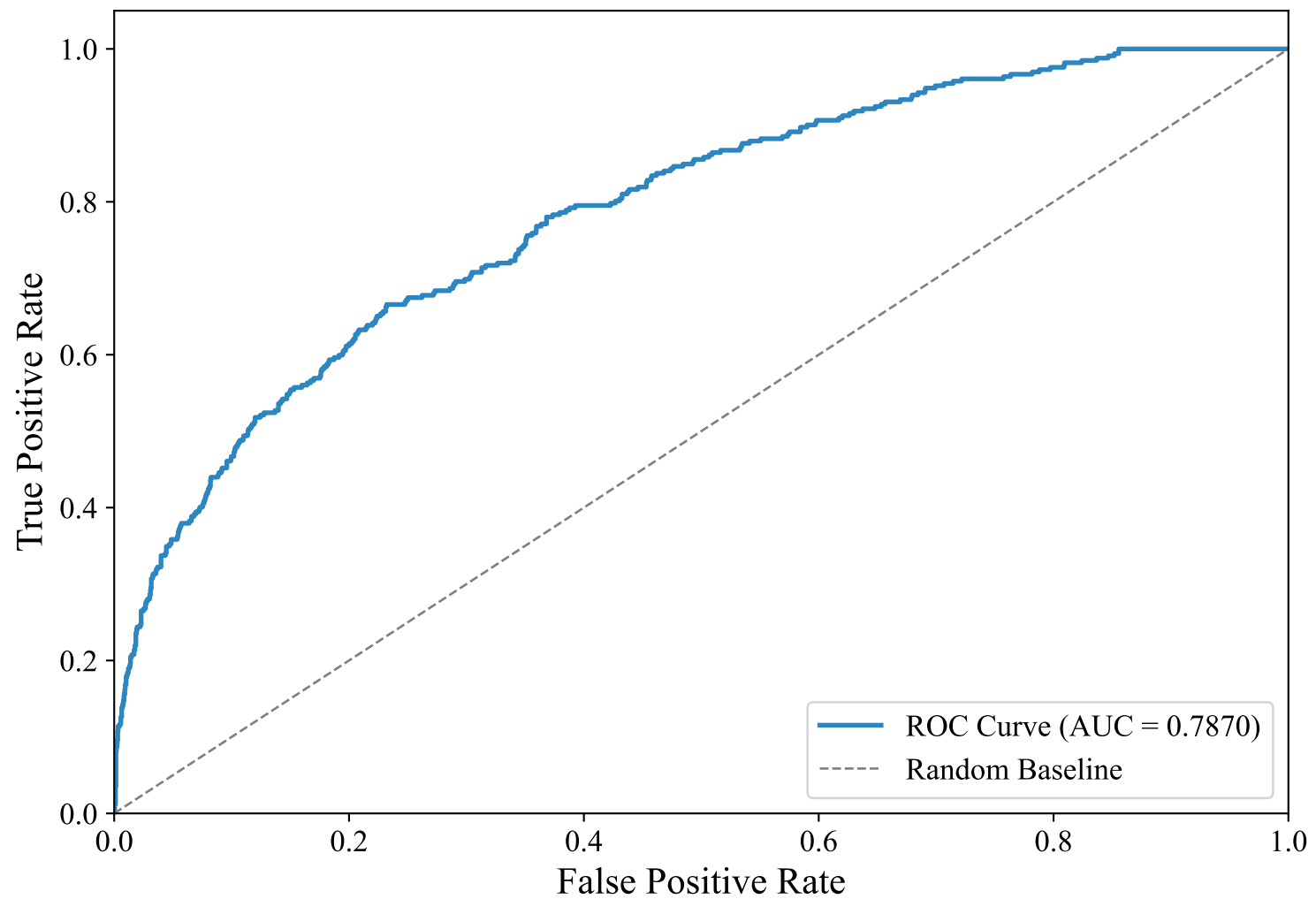
ROC Curve — GERMAN_MANUAL (efederici/e5-base-multilingual-4096, Random_Forest)
