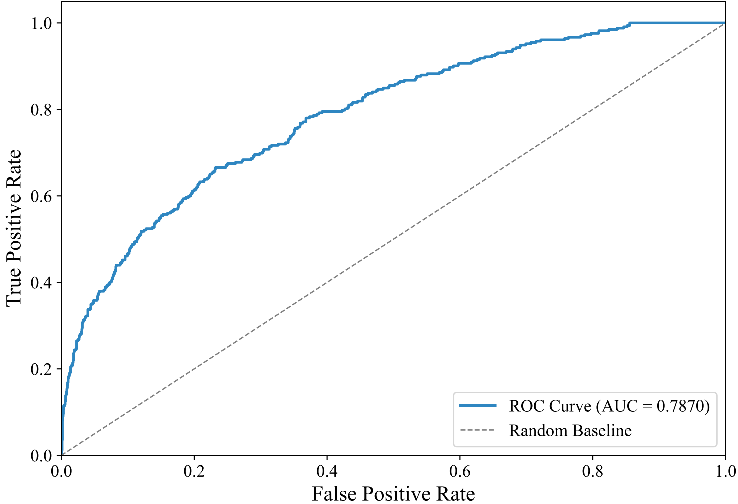
ROC Curve — GERMAN_MANUAL (efederici/e5-base-multilingual-4096, Random_Forest_Optimized)
